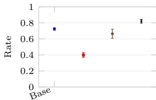
Abandon Rate
