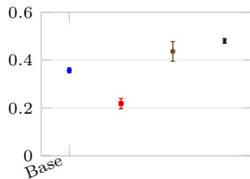
Helplessness \Delta
