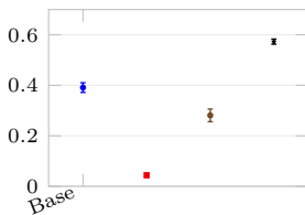
Negative Share
