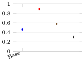
Negative Share
