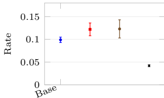
Abandon Rate
