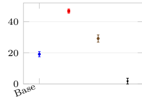
Helplessness \Delta
