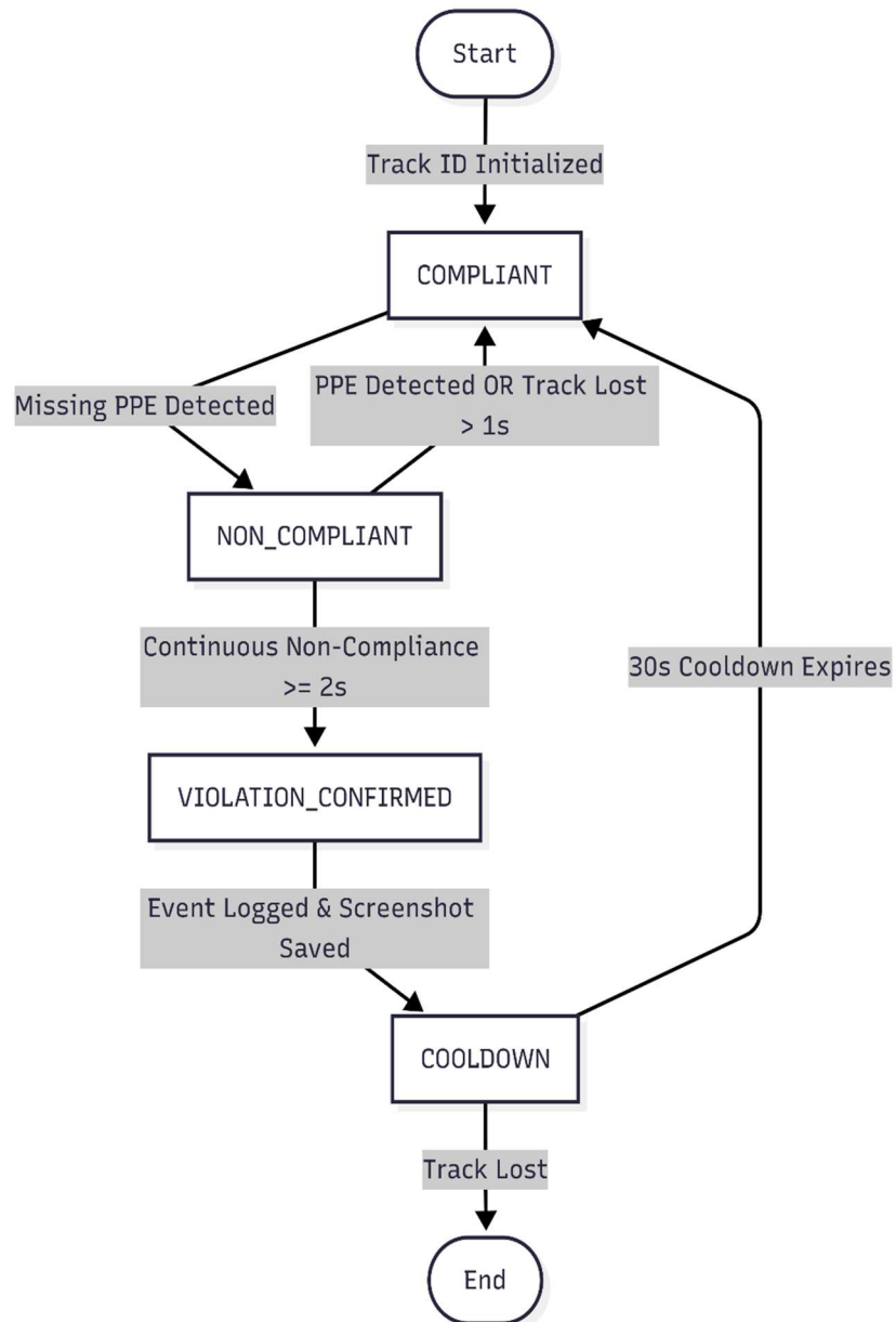
Diagram 3 – State Diagram
