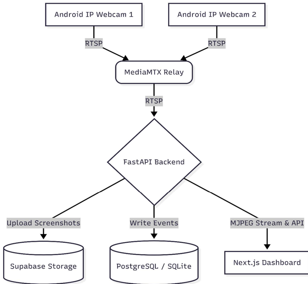
Diagram 1-System Context Diagram
