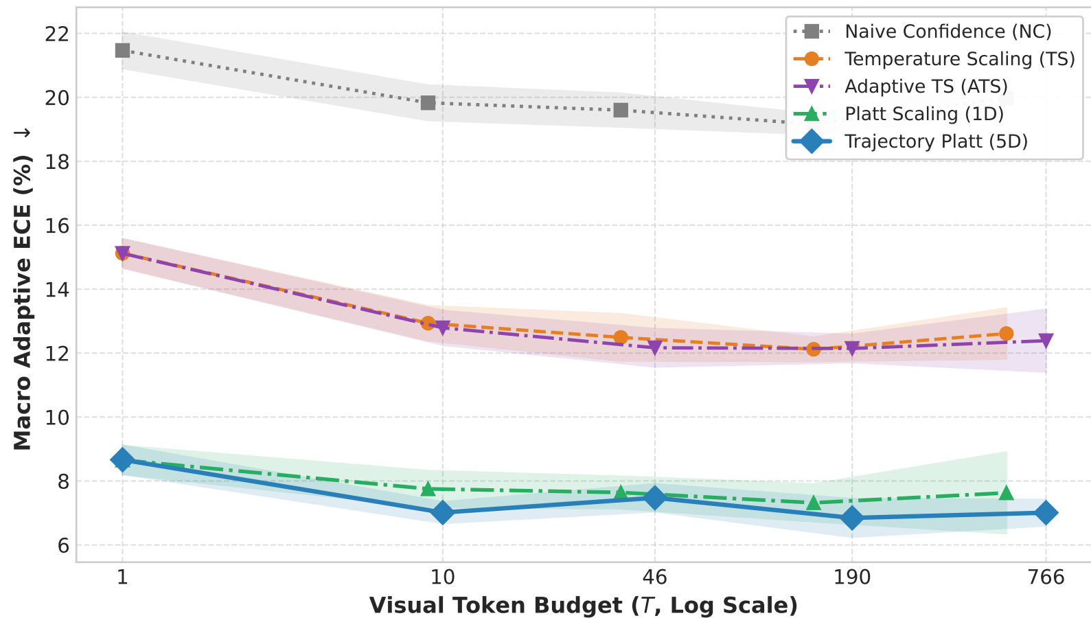
Visual Token Budget vs. Calibration Efficiency (M3-LLaVA 7B) Macro Average Across Core 5 Vision-Language Benchmarks
