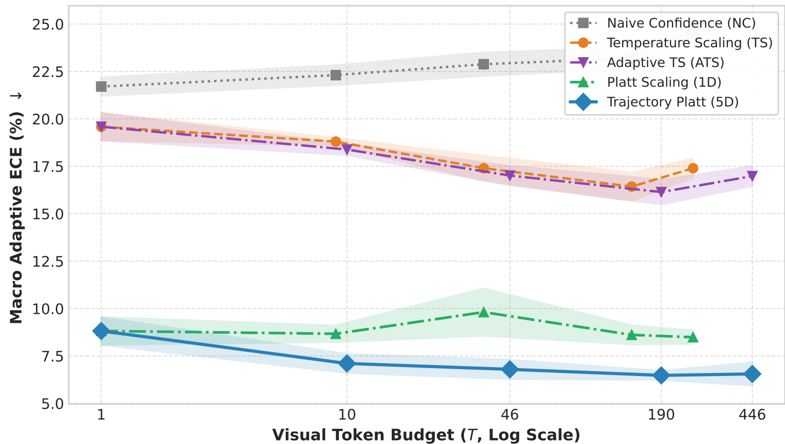
Visual Token Budget vs. Calibration Efficiency (MQT-LLaVA 7B) Macro Average Across Core 5 Vision-Language Benchmarks
