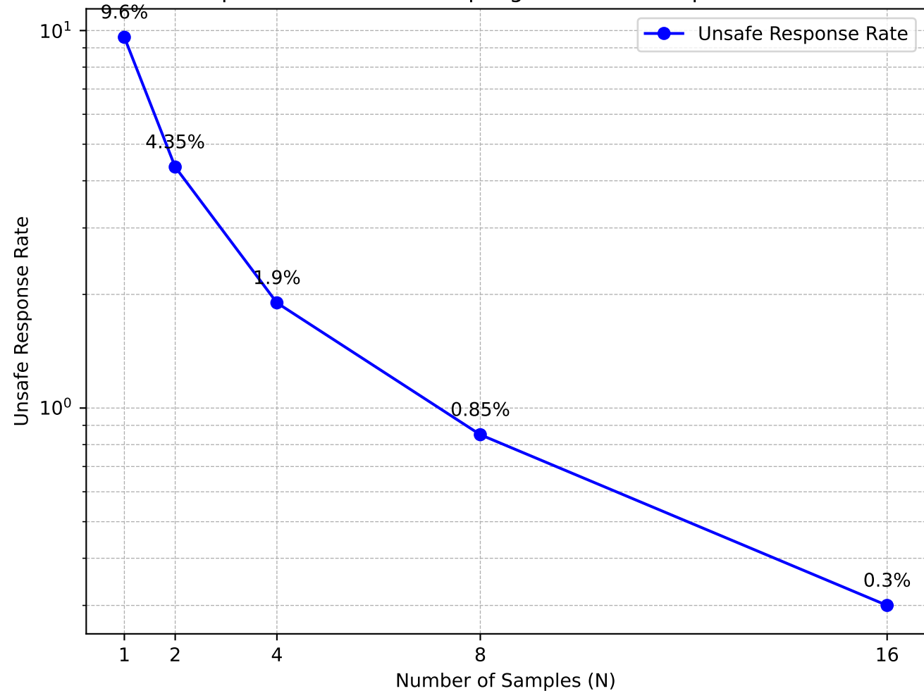
Impact of Best-of-N Sampling on Unsafe Response Rate
