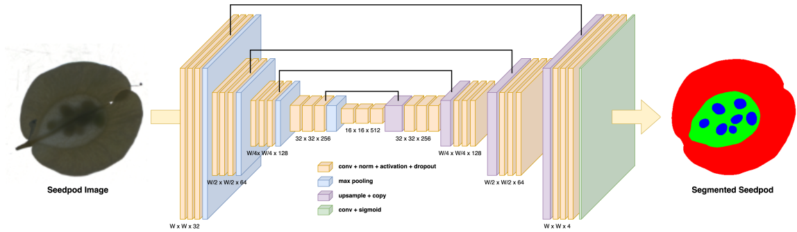
Figure 2.5: Pennycress U-Net architecture
