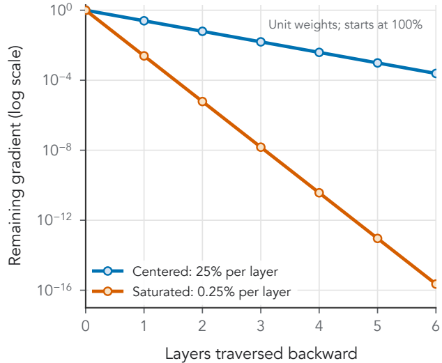
B Gradients vanish with depth
