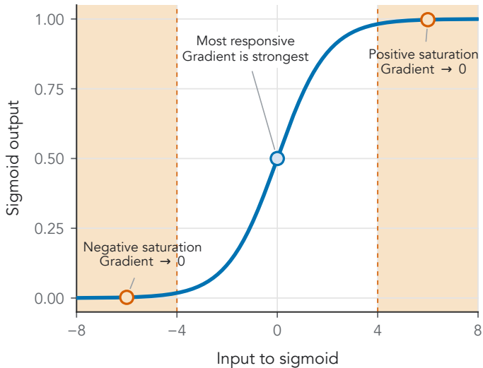
A Sigmoid saturation
