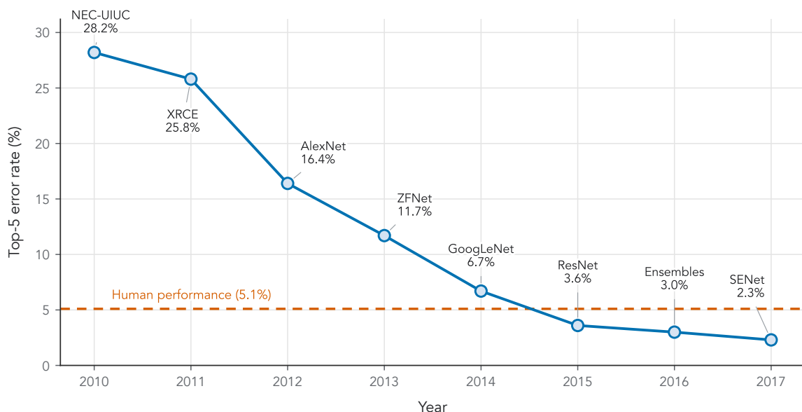
Figure 1.3: Winning top-5 classification error in the ImageNet Large Scale Visual Recognition Challenge (ILSVRC), 2010–2017. Points identify the best-performing entry in each year; the dashed line marks the reported 5.1% human baseline. The sharp decline after AlexNet in 2012 and subsequent gains from GoogLeNet, ResNet, model ensembles, and SENet show the rapid saturation of the benchmark.
