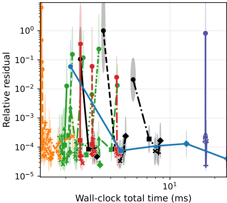
Synthetic Low-Rank + noise ( d=131072 , n=512 ) Sketch-and-ridge-regression
