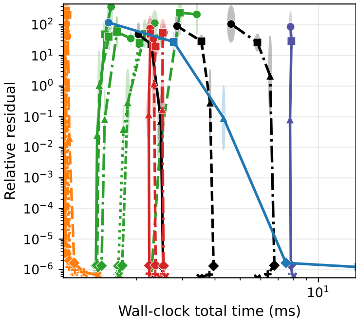
Synthetic Gaussian ( d=131072 , n=512 ) Sketch-and-ridge-regression
