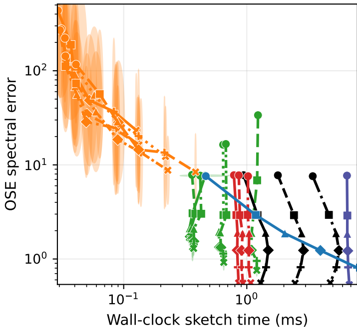
SuiteSparse - spal_004 ( d=131072 , n=512 ) OSE Spectral Error
