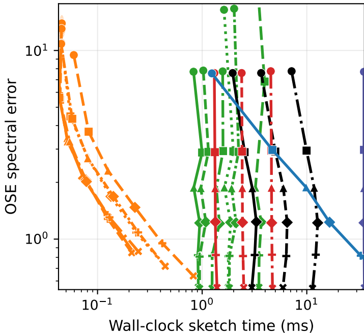
Synthetic Gaussian ( d=262144 , n=512 ) OSE Spectral Error
