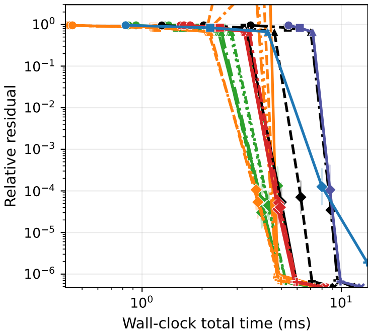
GPT2-medium stacked weights ( d=65536 , n=1024 ) Sketch+Solve
