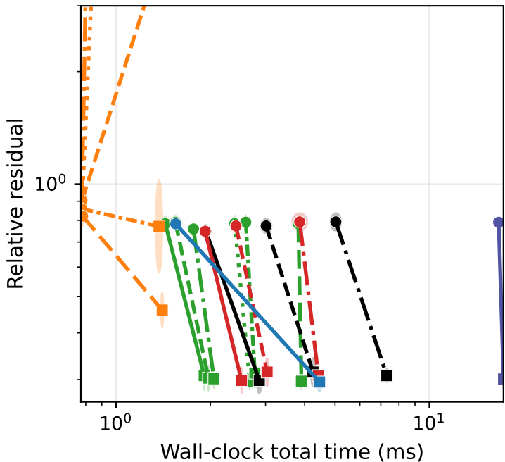
SuiteSparse - spal_004 (d=131072, n=512) Sketch+Solve
