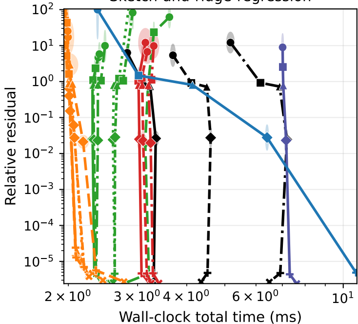
GPT2-medium stacked weights ( d=65536 , n=1024 ) Sketch-and-ridge-regression
