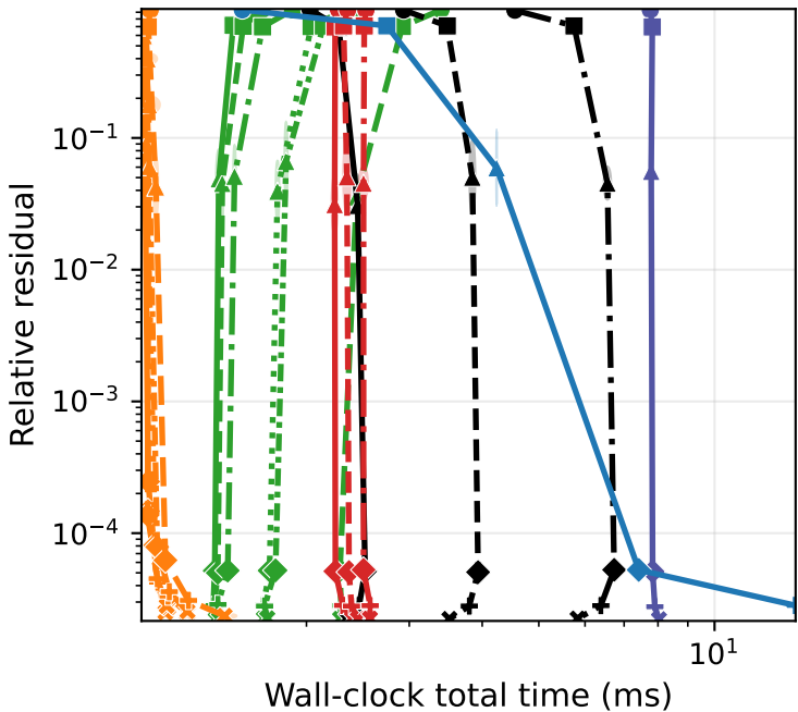
Qwen2-1.5B stacked weights ( d=131072 , n=512 ) Sketch-and-ridge-regression
