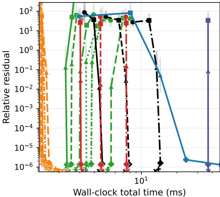
Synthetic Gaussian ( d=262144 , n=512 ) Sketch-and-ridge-regression
