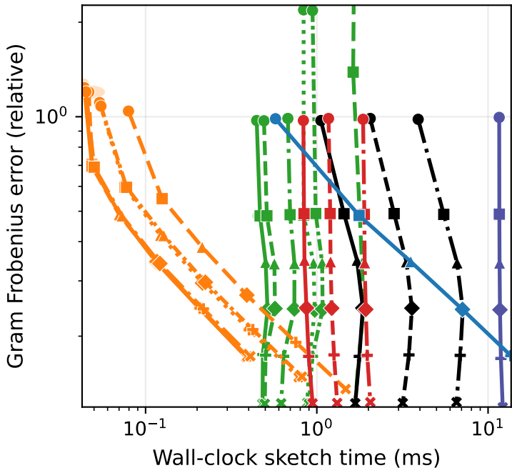
Synthetic Low-Rank + noise ( d=65536 , n=1024 ) Gram Matrix Approximation
