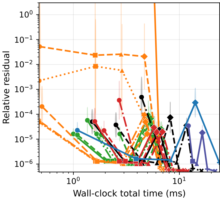
Synthetic Low-Rank + noise ( d=65536 , n=1024 ) Sketch+Solve
