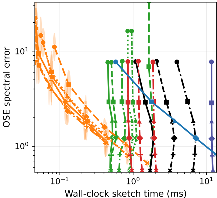
Synthetic Low-Rank + noise ( d=65536 , n=1024 ) OSE Spectral Error
