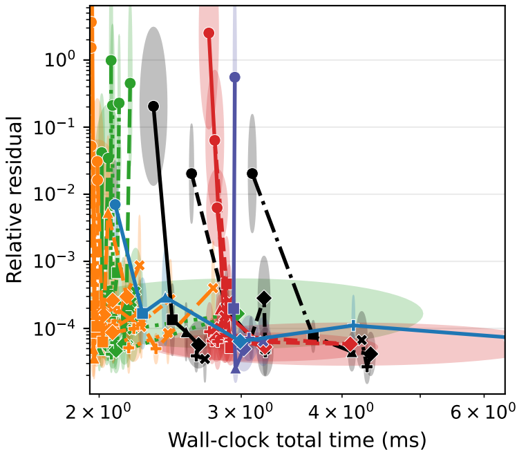
Synthetic Low-Rank + noise ( d=16384 , n=1024 ) Sketch-and-ridge-regression
