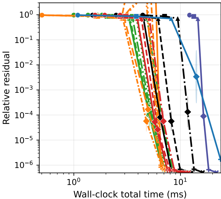
Synthetic Gaussian ( d=65536 , n=1024 ) Sketch+Solve
