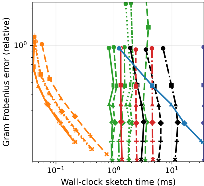
Synthetic Low-Rank + noise ( d=262144 , n=512 ) Gram Matrix Approximation
