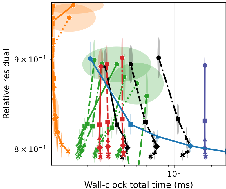
SuiteSparse - spal_004 (d=262144, n=512) Sketch-and-ridge-regression
