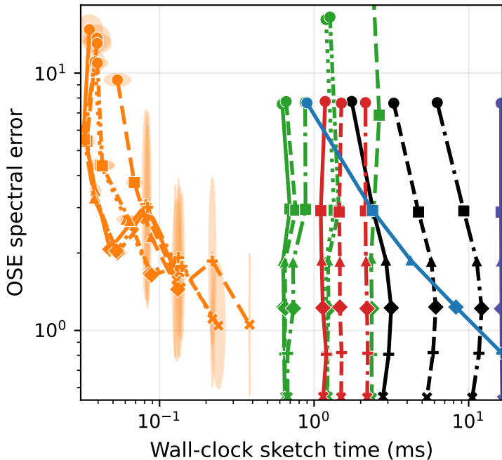
Synthetic Low-Rank + noise ( d=262144 , n=512 ) OSE Spectral Error
