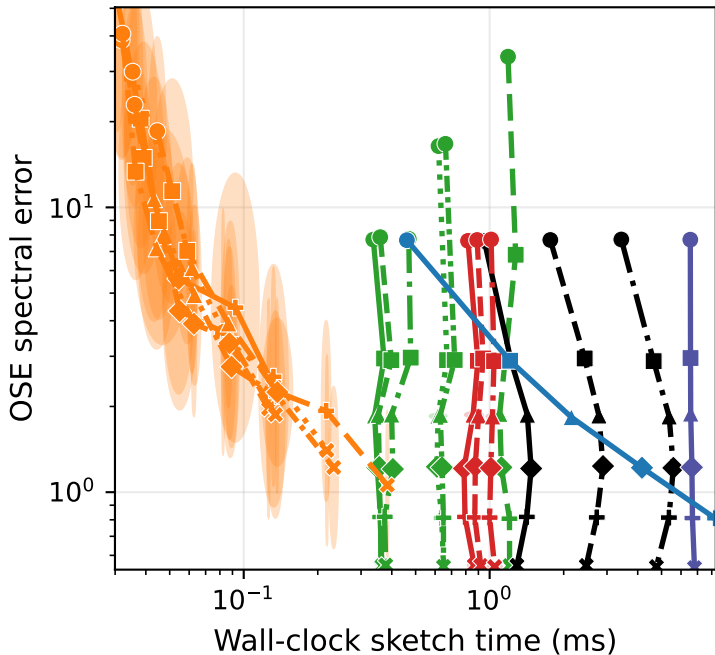
Synthetic Low-Rank + noise ( d=131072 , n=512 ) OSE Spectral Error
