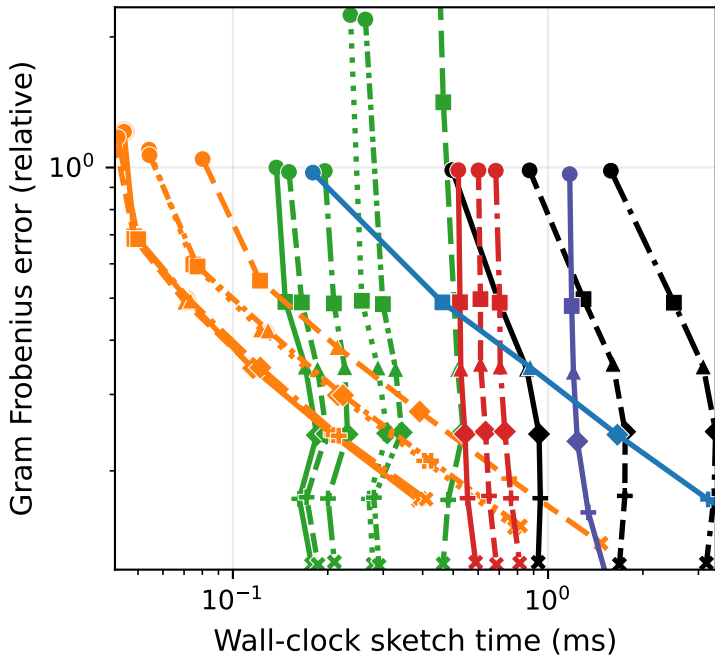
Synthetic Low-Rank + noise ( d=16384 , n=1024 ) Gram Matrix Approximation
