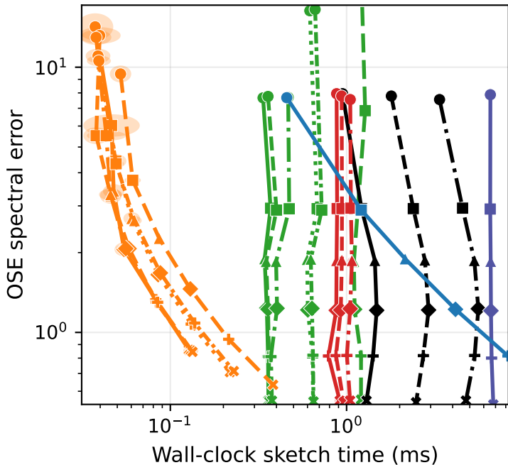
Synthetic Gaussian ( d=131072 , n=512 ) OSE Spectral Error
