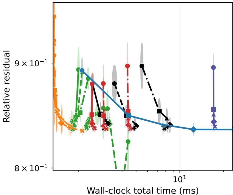
SuiteSparse - spal_004 ( d=131072 , n=512 ) Sketch-and-ridge-regression
