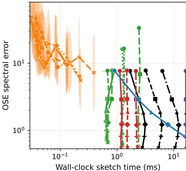
SuiteSparse - spal_004 ( d=262144 , n=512 ) OSE Spectral Error
