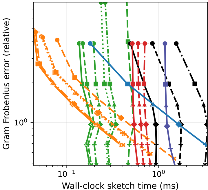
Synthetic Gaussian ( d=16384 , n=1024 ) Gram Matrix Approximation
