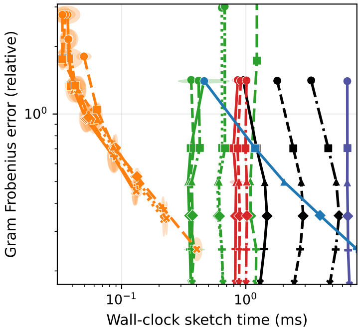
SuiteSparse - spal_004 ( d=131072 , n=512 ) Gram Matrix Approximation
