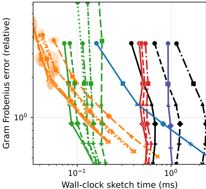
GPT2-medium stacked weights ( d=16384 , n=1024 ) Gram Matrix Approximation
