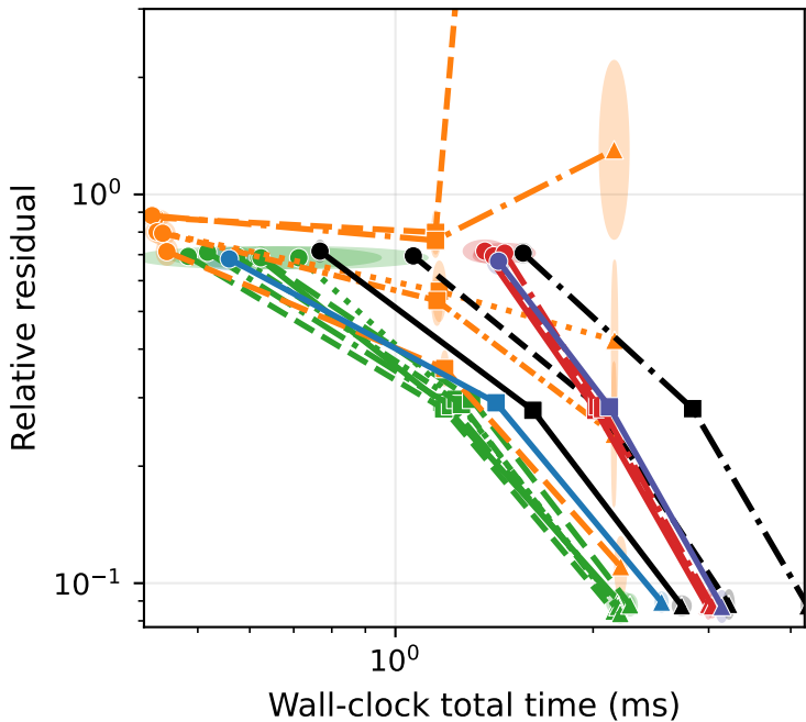
SuiteSparse - spal_004 (d=16384, n=1024) Sketch+Solve
