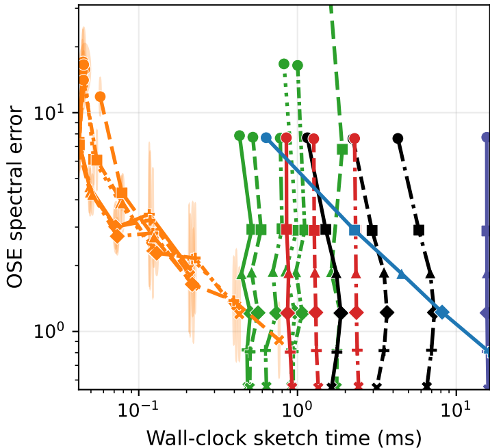
Qwen2-1.5B stacked weights ( d=131072 , n=512 ) OSE Spectral Error
