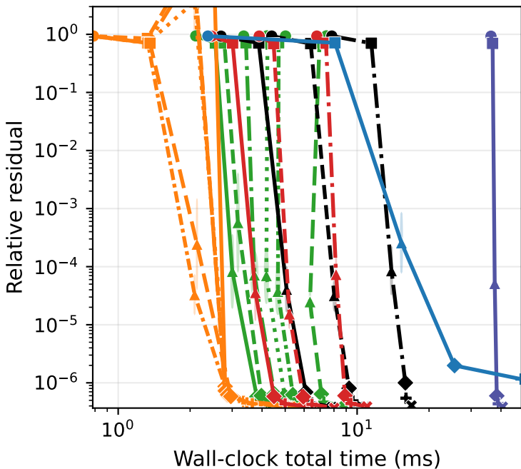
Synthetic Gaussian ( d=262144 , n=512 ) Sketch+Solve
