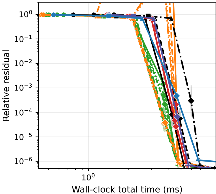
GPT2-medium stacked weights ( d=16384 , n=1024 ) Sketch+Solve
