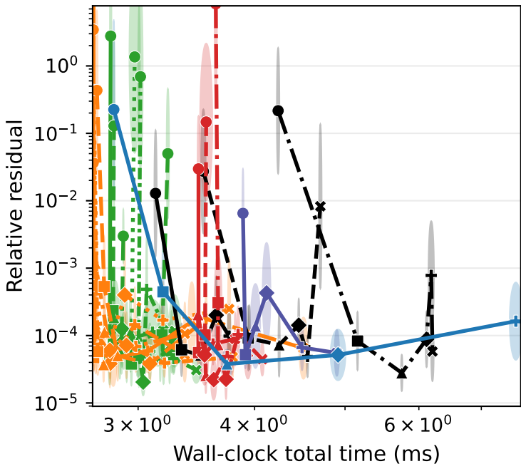
Synthetic Low-Rank + noise ( d=16384 , n=1024 ) Sketch-and-ridge-regression
