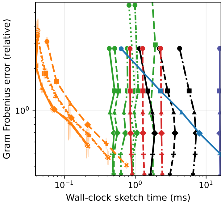
Qwen2-1.5B stacked weights ( d=131072 , n=512 ) Gram Matrix Approximation
