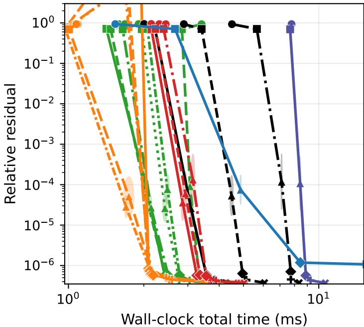
Qwen2-1.5B stacked weights ( d=131072 , n=512 ) Sketch+Solve
