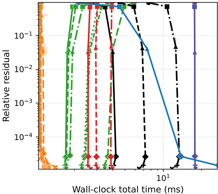
Qwen2-1.5B stacked weights ( d=262144 , n=512 ) Sketch-and-ridge-regression
