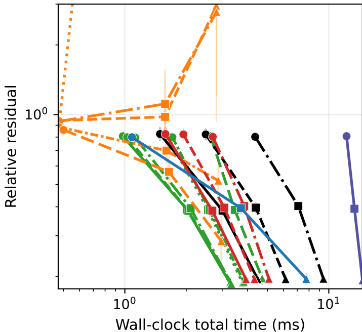
SuiteSparse - spal_004 (d=65536, n=1024) Sketch+Solve
