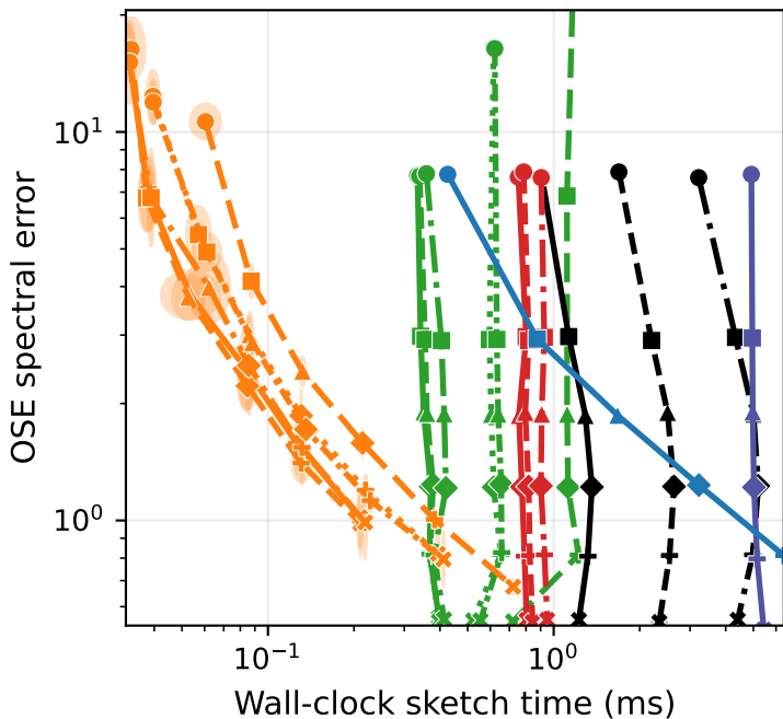
GPT2-medium stacked weights ( d=65536 , n=1024 ) OSE Spectral Error
