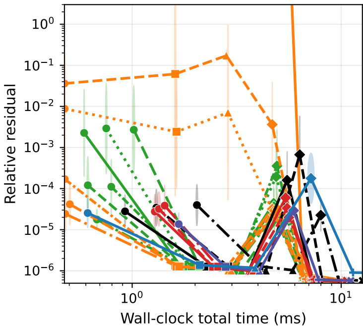
Synthetic Low-Rank + noise ( d=16384 , n=1024 ) Sketch+Solve
