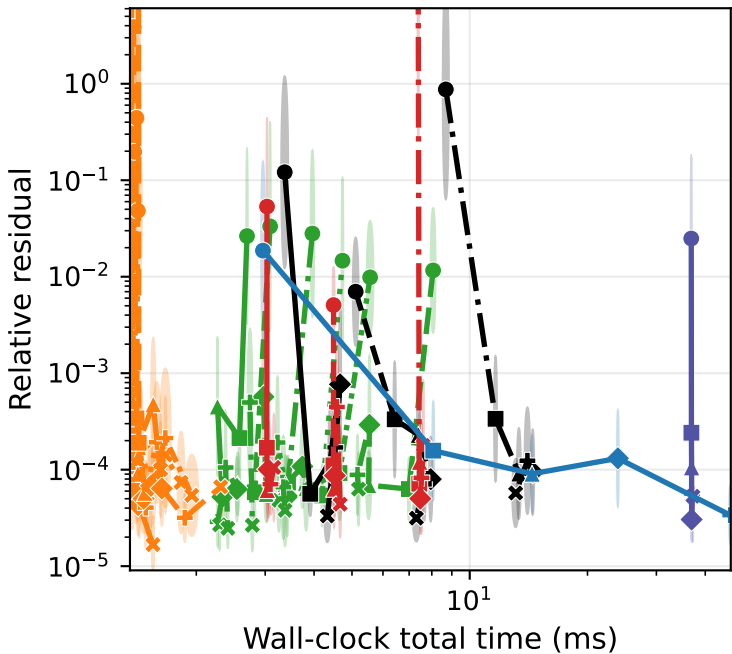
Synthetic Low-Rank + noise ( d=262144 , n=512 ) Sketch-and-ridge-regression
