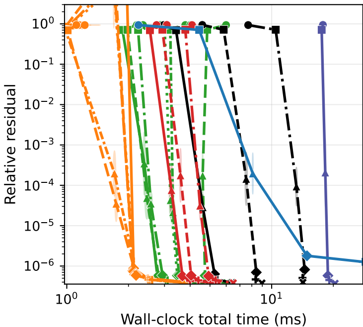
Qwen2-1.5B stacked weights ( d=262144 , n=512 ) Sketch+Solve
