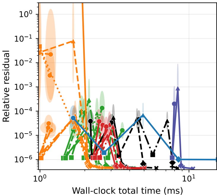
Synthetic Low-Rank + noise ( d=131072 , n=512 ) Sketch+Solve
