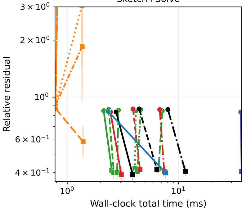
SuiteSparse - spal_004 ( d=262144 , n=512 ) Sketch+Solve
