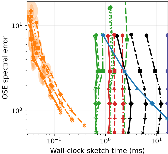
Qwen2-1.5B stacked weights ( d=262144 , n=512 ) OSE Spectral Error
