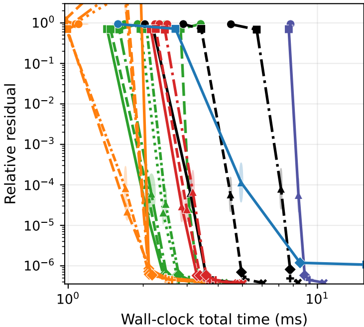
Synthetic Gaussian ( d=131072 , n=512 ) Sketch+Solve
