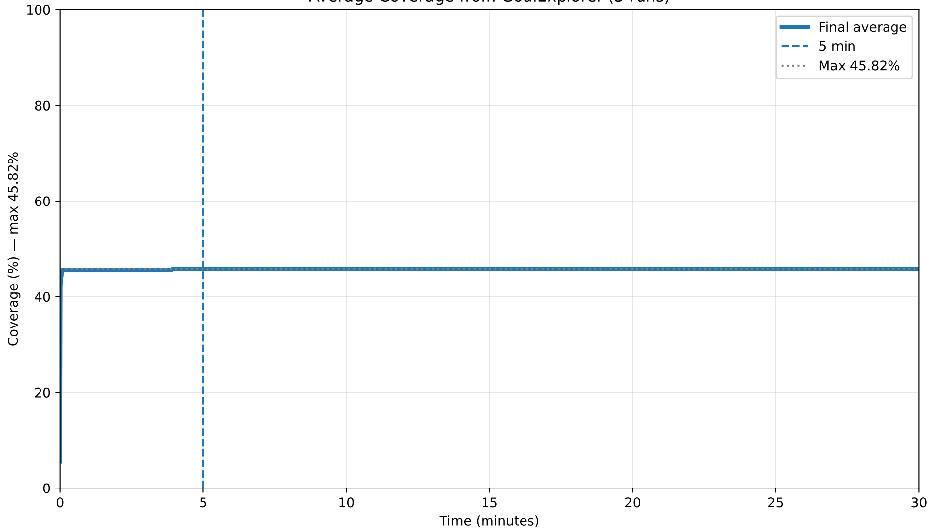
Average Coverage from GoalExplorer (3 runs)
