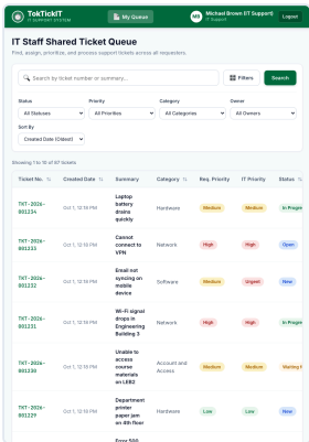
Figure 6.2: Staff Queue on Tablet (820x1180)
