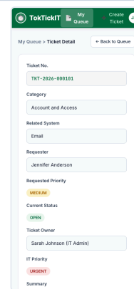
Figure 7.4: Ticket Detail on Mobile (390x844)
