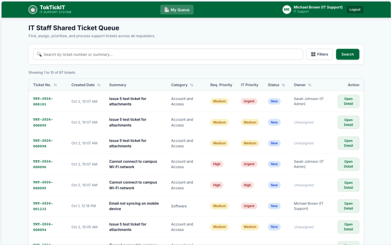
Figure 6.1: Shared IT Staff Ticket Queue (Desktop, 1440x900) — Search, multi-select filters, priority badges, Open Detail
