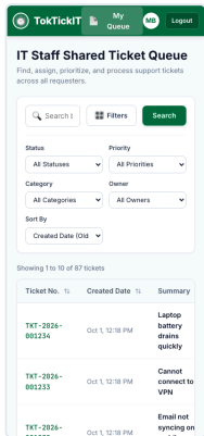
Figure 6.3: Staff Queue on Mobile (390x844)
