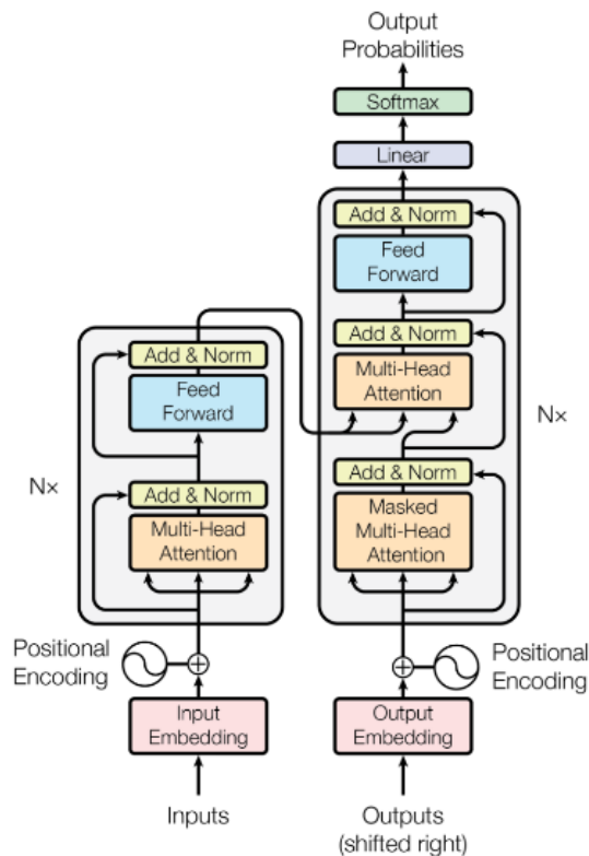
Figure 4.1: Overview of the Transformer architecture, as introduced in the paper *Attention is All You Need* vaswani2017attention
