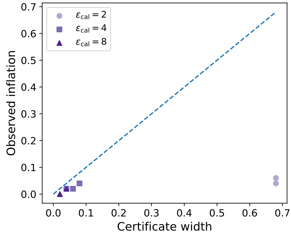
Observed inflation vs certificate
