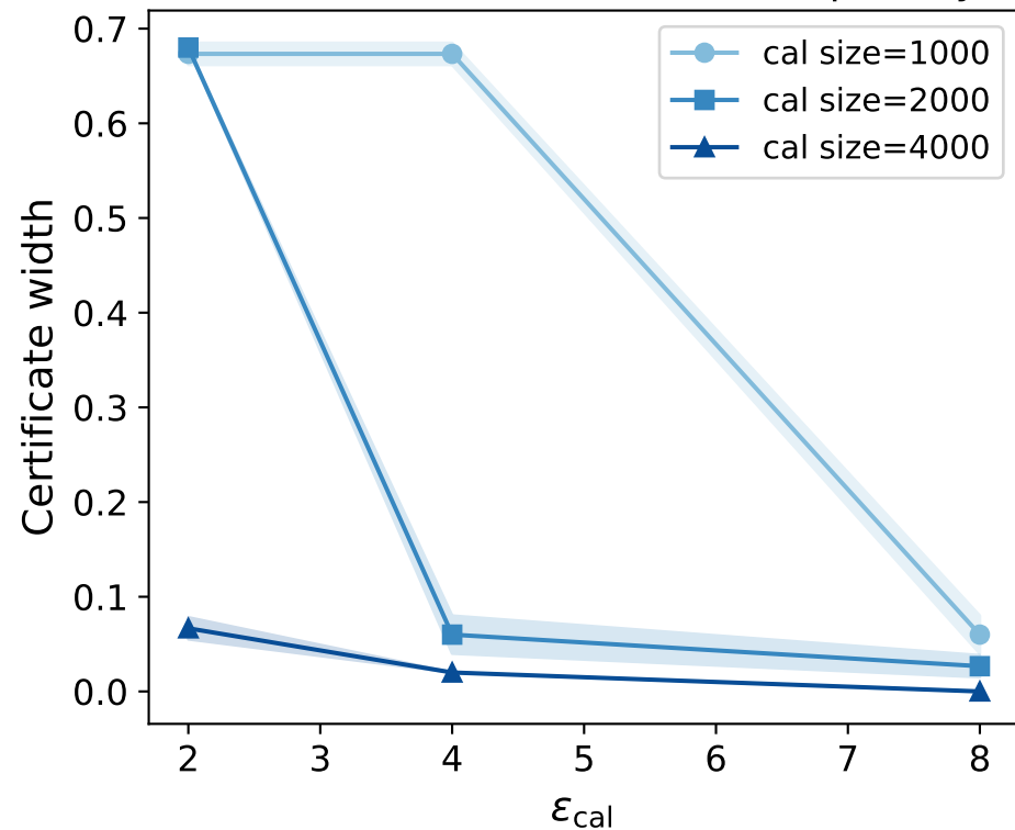
Certificate width vs calibration privacy
