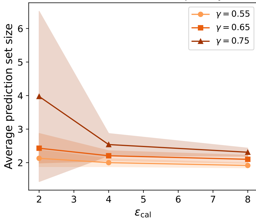
Set size vs calibration privacy
