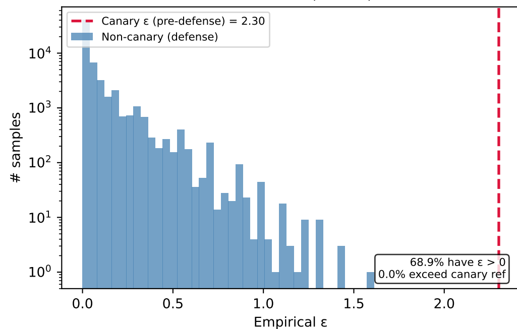
CP no holdout (inflated)
