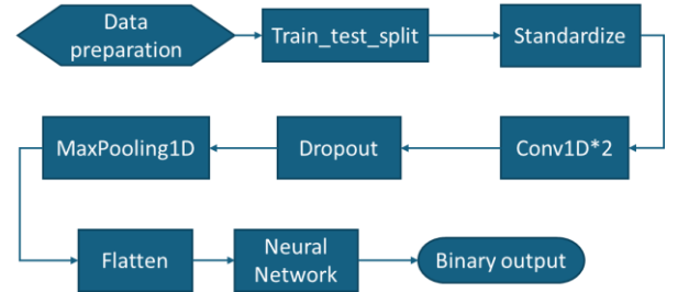
Fig. 9. Flow of 1D-CNN.
