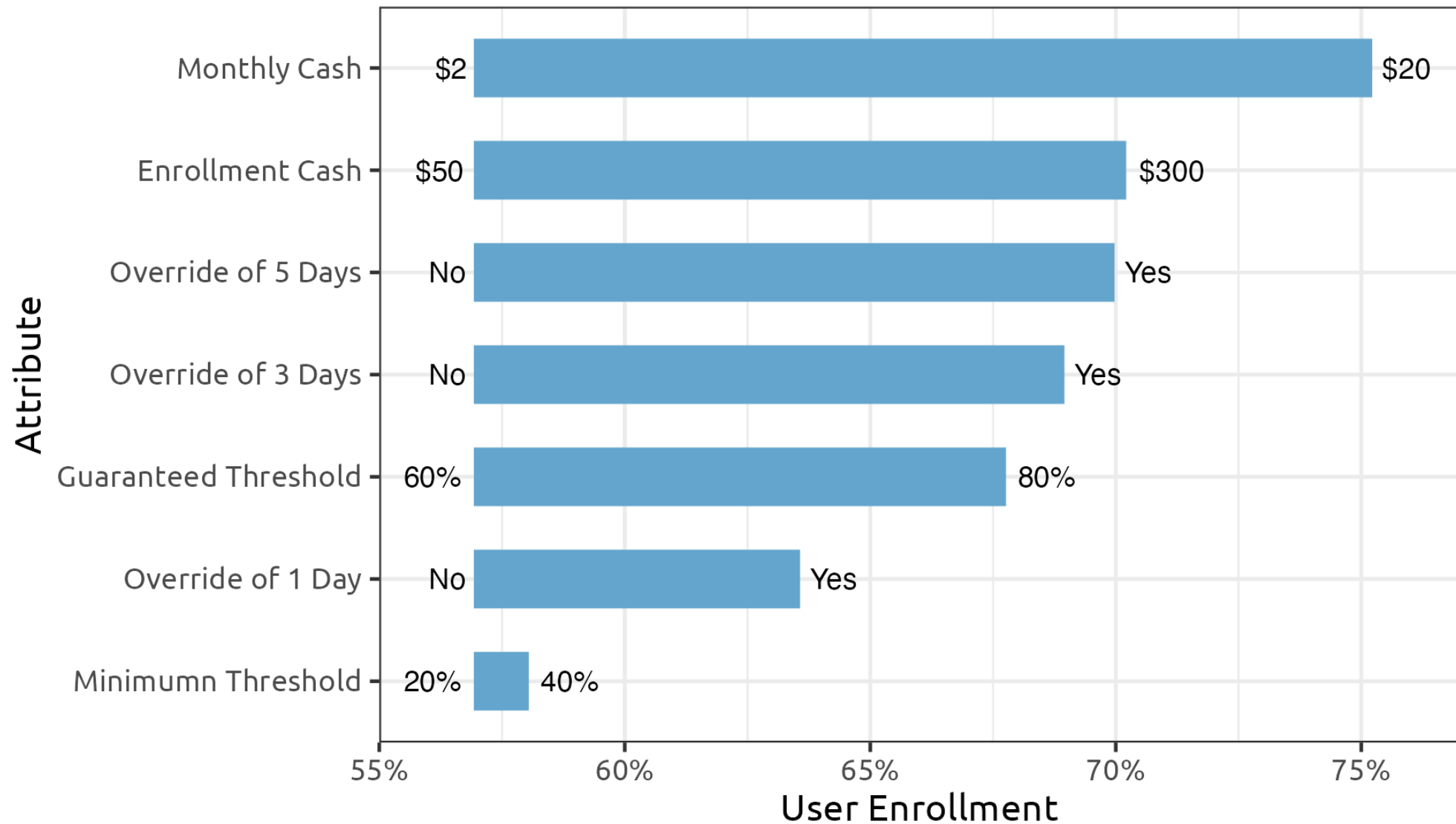
SMC Enrollment Sensitivity Plots - Combined
