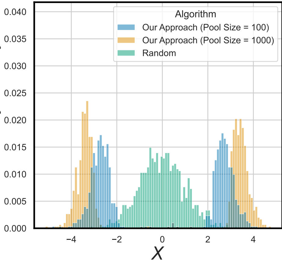
Probability Density
