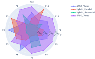
Algorithm Performance Ranking (20D) - Closer to Center is Better
