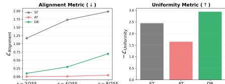
Figure 3: Representation metrics on CIFAR-10 for the standard-trained model (ST), the adversarially trained model (AT), and the diffusion representations (DR).
