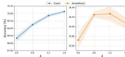
Figure 6: Clean and Robust accuracy on CIFAR-100 for DM-AT+DRA with different DRA regularization strength \lambda .
