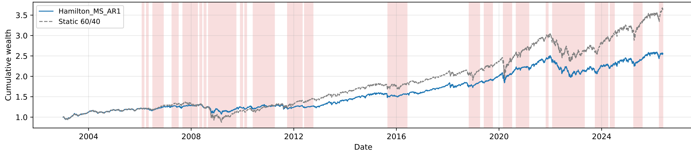
Cumulative wealth: Hamilton_MS_AR1 vs Static 60/40 (red shading = risk-off periods)
