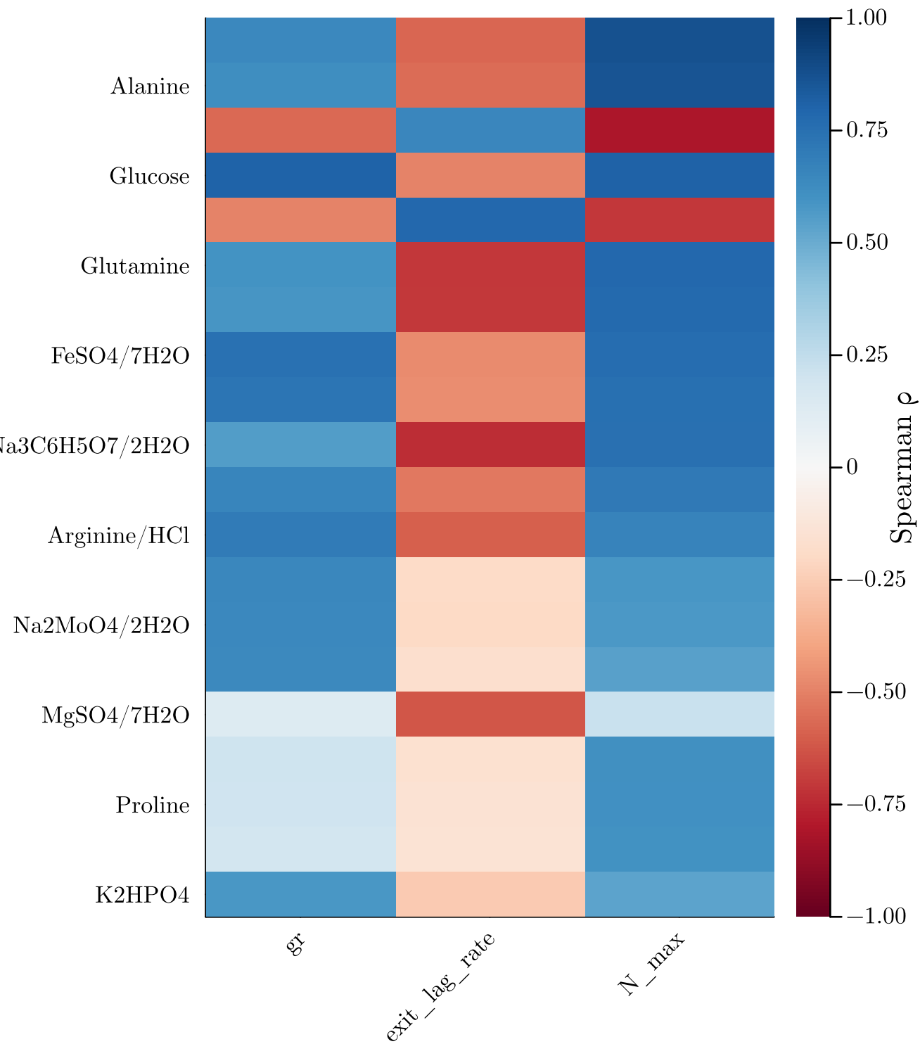
Figure 3: Top 20 Compounds - Correlation Heatmap
