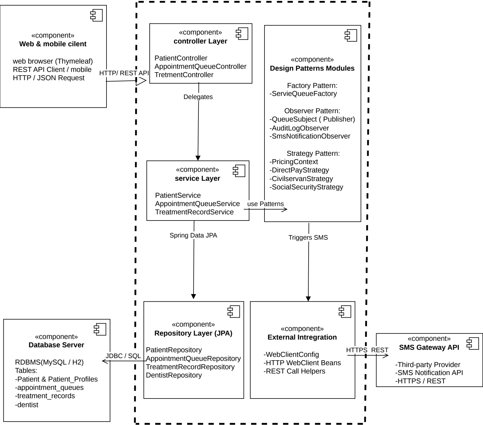
Component Diagram
