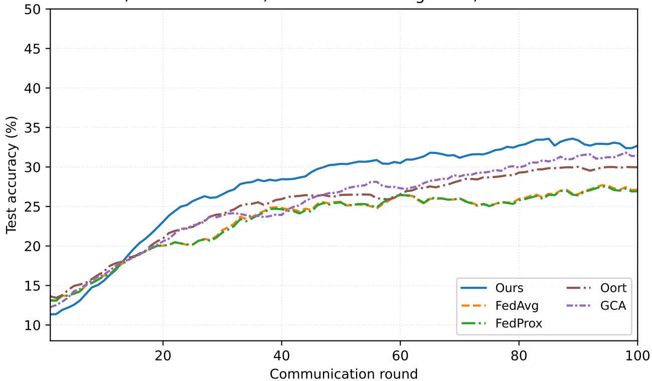
CIFAR-10, Dirichlet \alpha = 0.1 , channel-noise diagnostic, mean over 3 seeds
