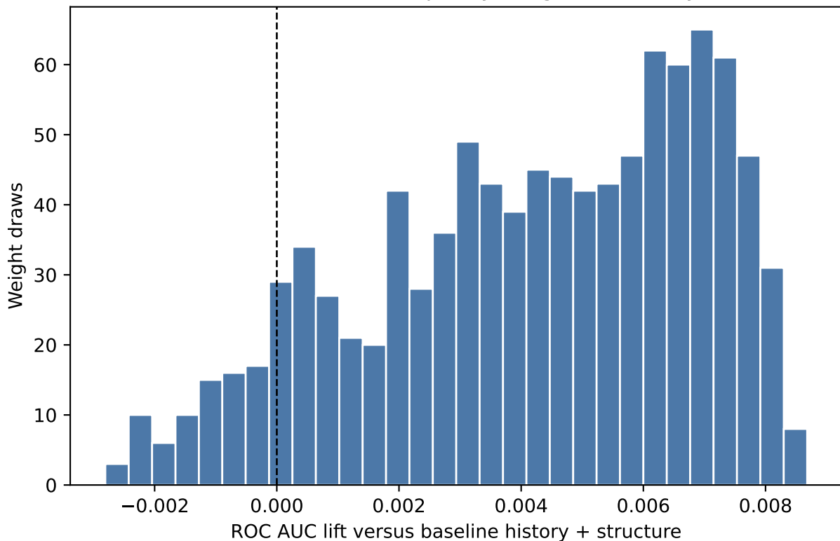
File-level holdout opacity-weight sensitivity
