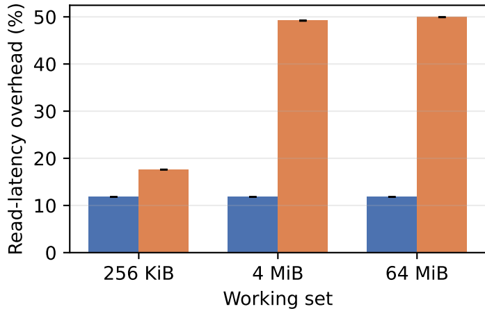
Request period 20 ns
