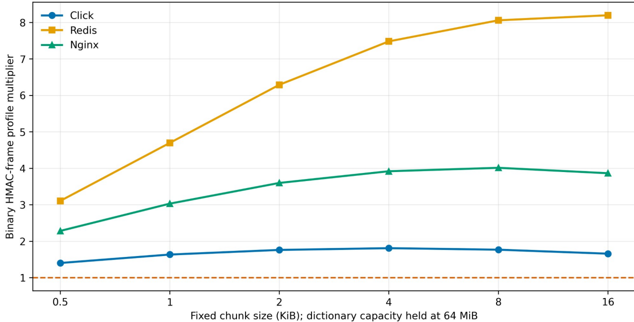
Figure 3. Named-object sensitivity to fixed chunk size with byte-equivalent 64 MiB dictionaries. All points reconstruct exactly.
