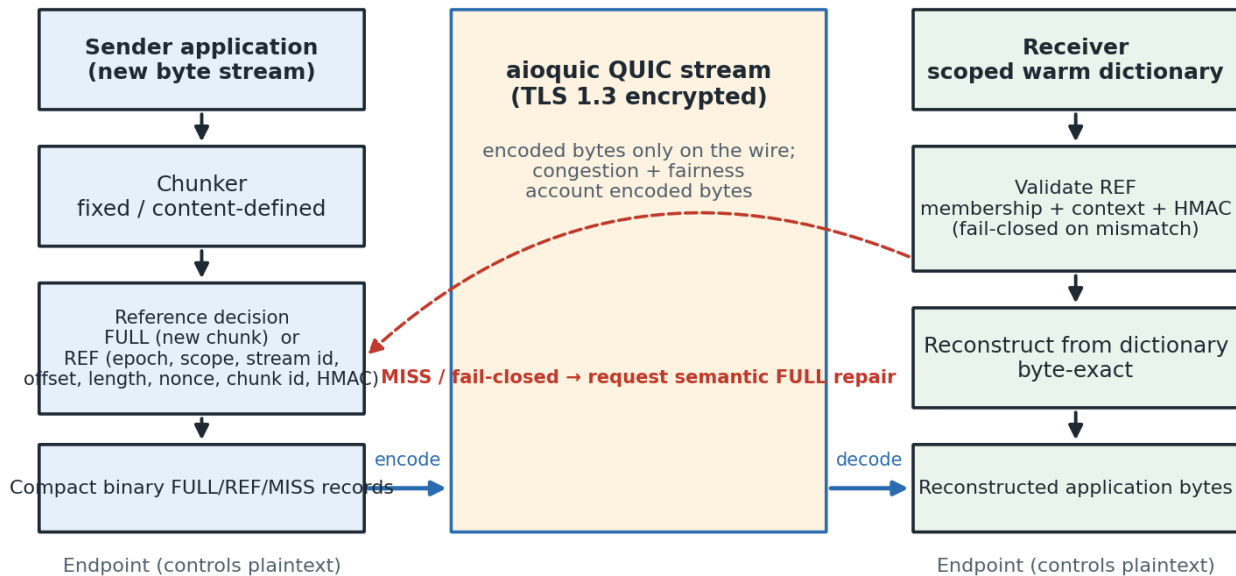
Figure 1. ReduLink protocol and deployment architecture. The sender chunks outgoing bytes and emits FULL or authenticated REF records carried as compact binary application data inside an encrypted QUIC stream; the receiver validates each reference against dictionary membership and bound context before byte-exact reconstruction, failing closed and requesting semantic FULL repair on any mismatch.
