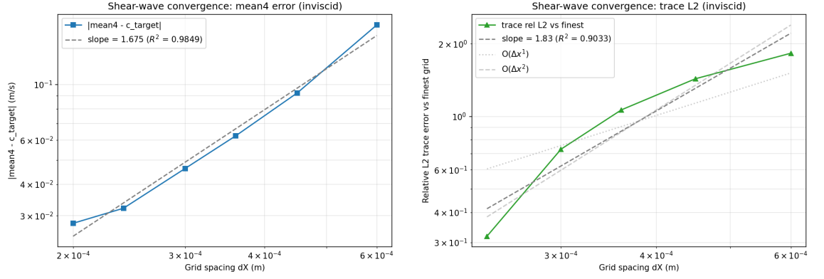
Figure 2. Grid convergence study. Left: Wavespeed convergence ( |\text{mean}_4 - c_{\text{target}}| ) vs grid spacing (log-log). Fitted slope 1.68, R^2 = 0.98 . Right: Trace L_2 convergence (relative L_2 error of velocity traces vs finest grid). Fitted slope 1.83, R^2 = 0.90 . Dashed reference lines show O(\Delta x) and O(\Delta x^2) .
