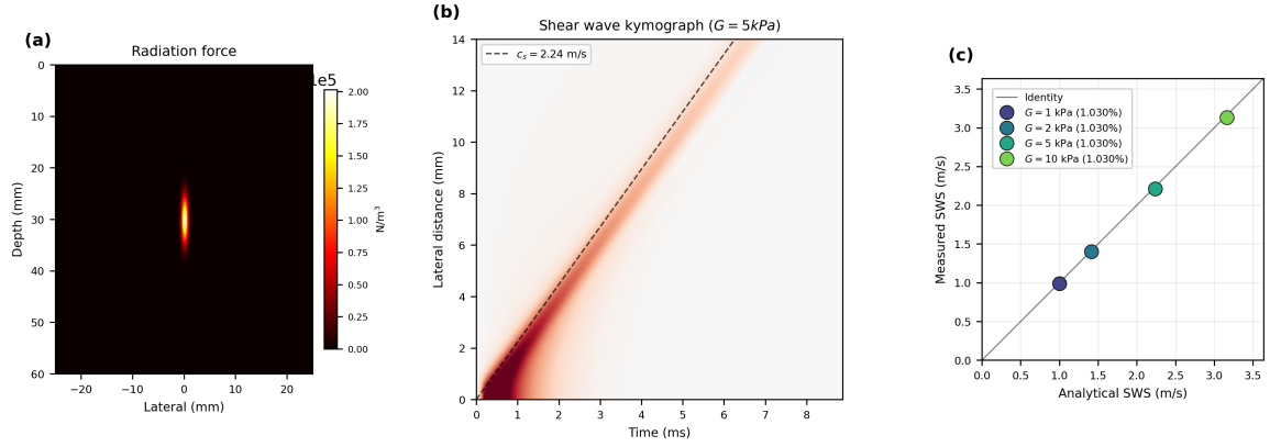
Figure 4. QIBA elastic phantom validation using a Gaussian body force excitation matching the QIBA GaussExc convention. (a) Gaussian radiation force distribution (Eq. 42), with the focal spot centered at 30 mm depth. (b) Space–time kymograph of axial displacement for the G = 5 kPa phantom; the dashed line indicates the analytical shear wave speed c_s = 2.24 m/s. (c) Recovered shear wave speed vs. analytical value for all four QIBA elastic phantoms ( G = 1 –10 kPa); all configurations recover the wavespeed to within \sim 1\% .
