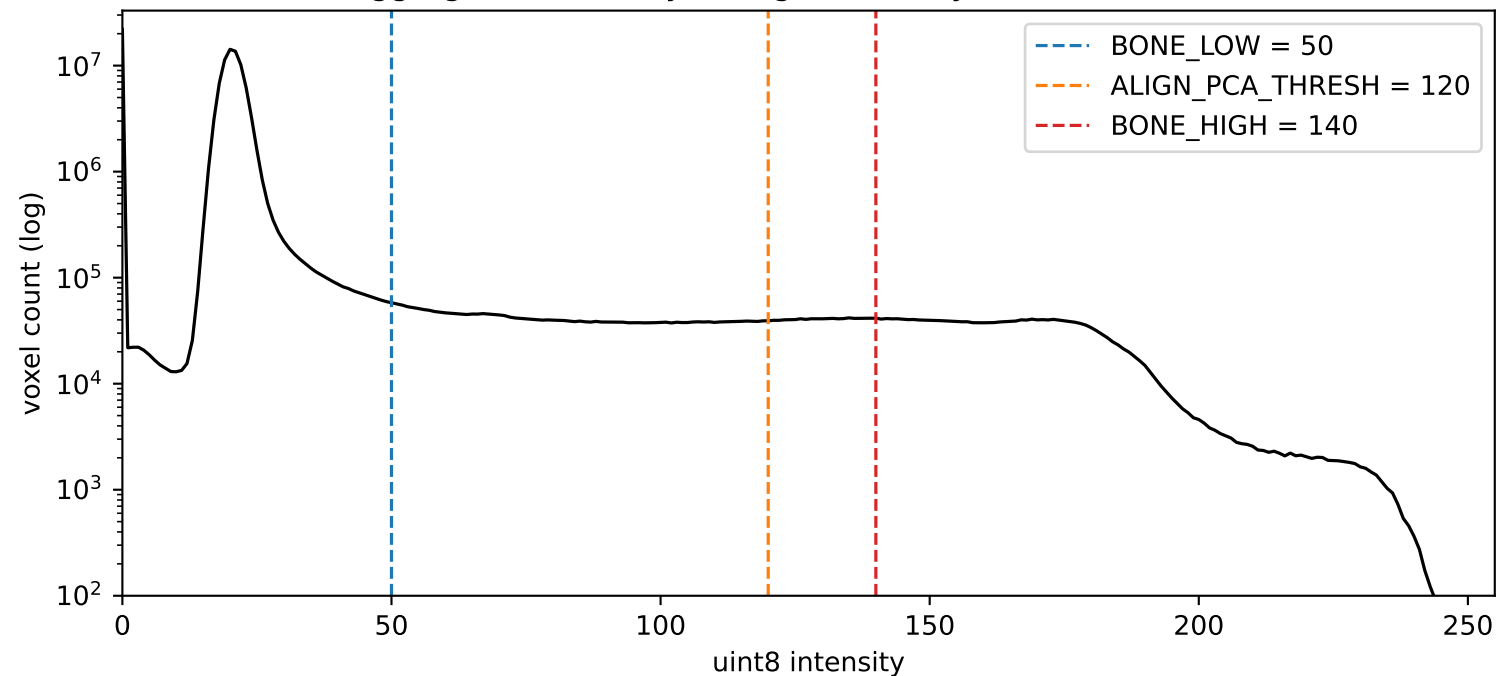
TMM M-2272 aggregated intensity histogram (every 16th slice, total 103.8M voxels)
