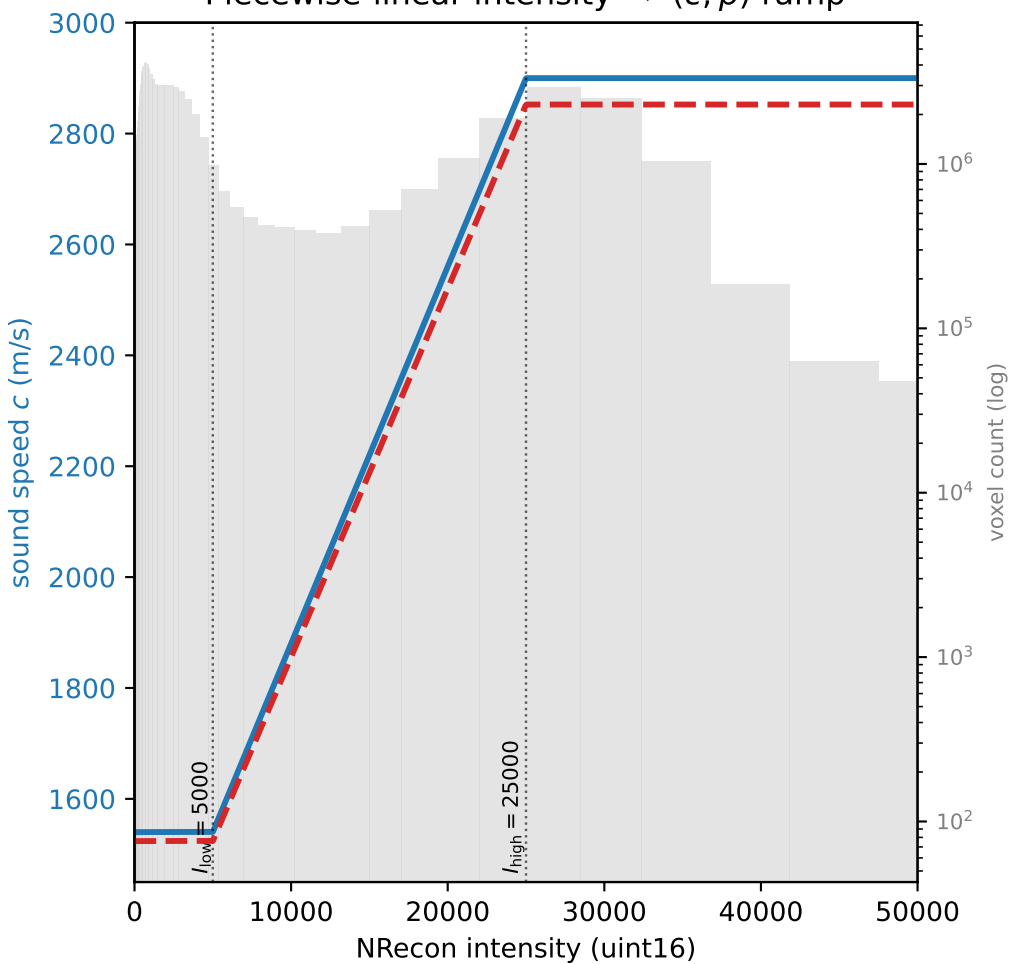
Piecewise-linear intensity \rightarrow (c, \rho) ramp
