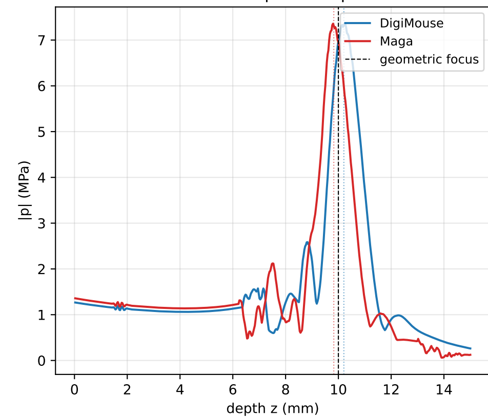
On-axis axial pressure profile
