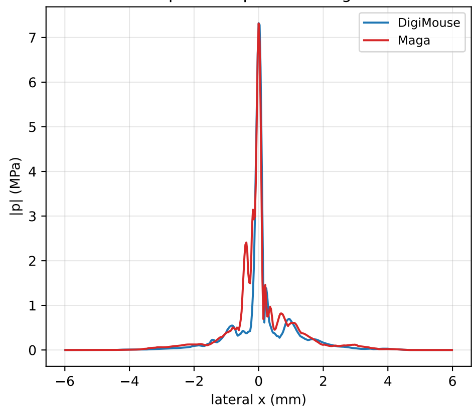
Lateral pressure profile through focus
