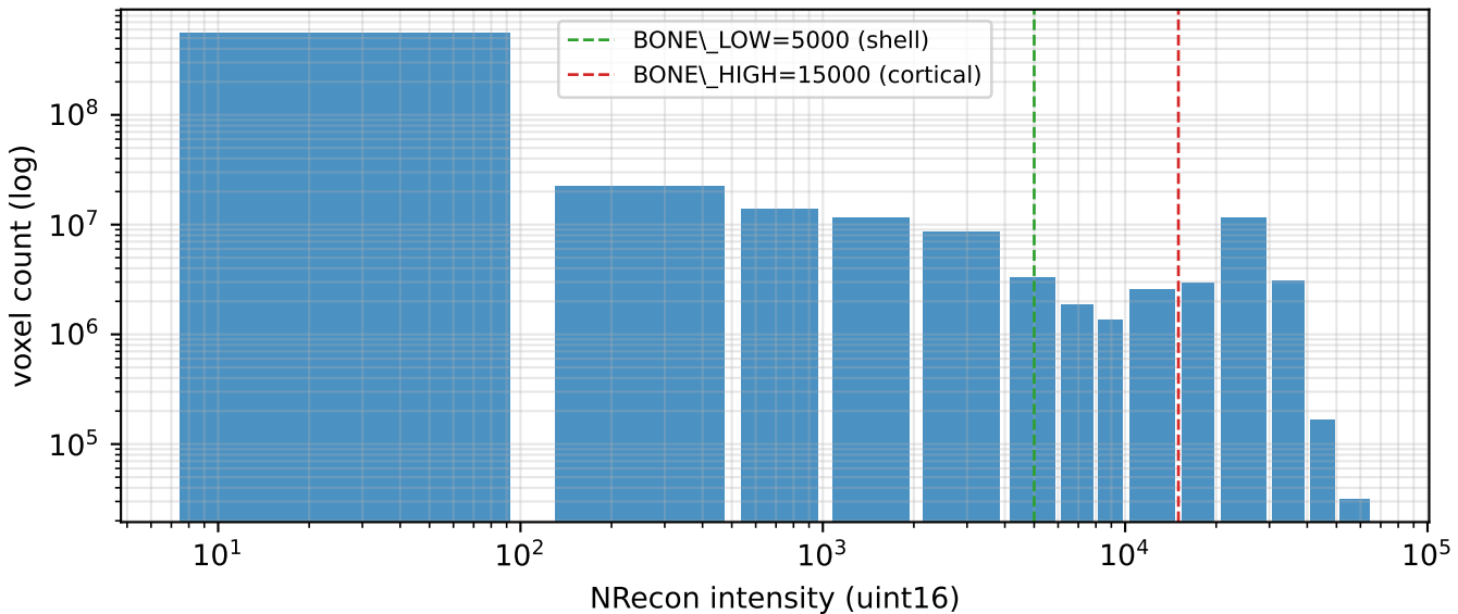
Maga 4K native (6.127 \mu\text{m} ): intensity histogram (0.6 G voxels)
