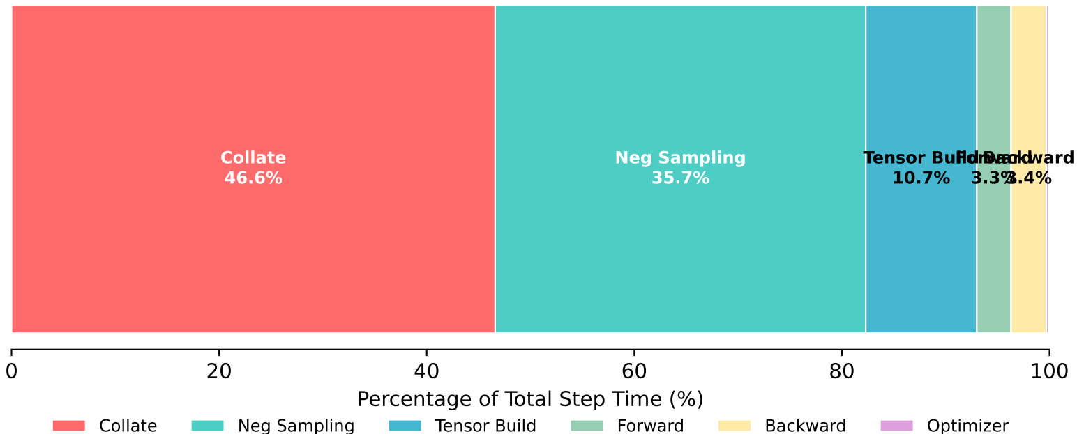
Fig 1: MuKG Training Step Profiling Breakdown
