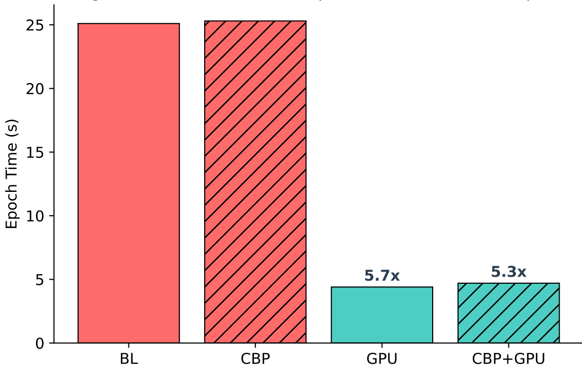
Fig 5: Main Benchmark — Epoch Time (Phase 9 Step 2)
