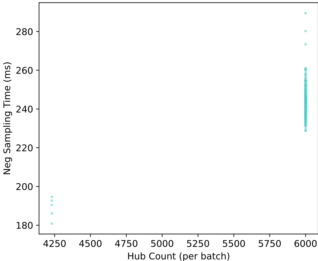
Fig 2: Cost Model Correlation ( R=0.701 )
