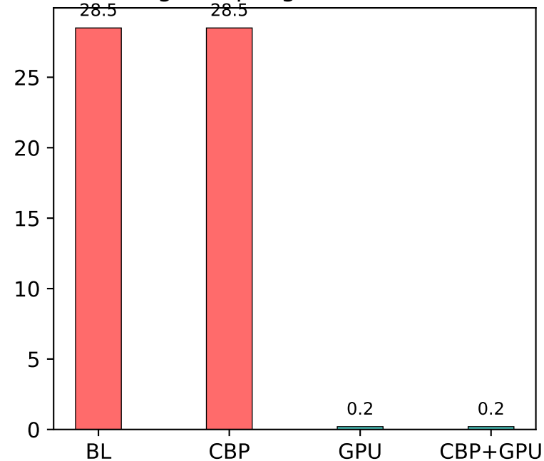
Fig 6: Ablation — Variance Comparison (Phase 9 Step 3, epoch 9)
