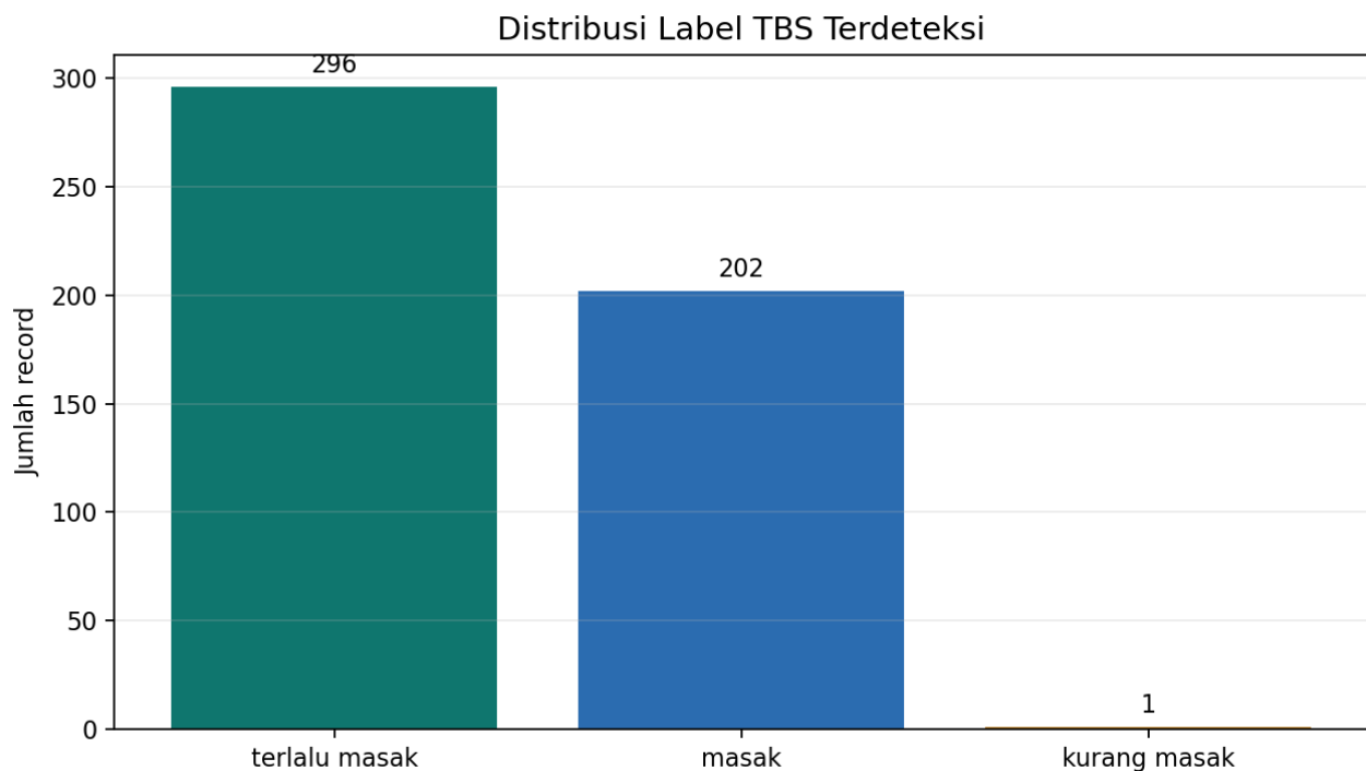
Distribusi label
