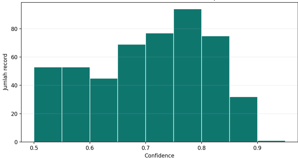
Histogram confidence
