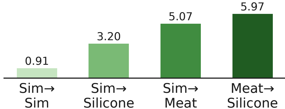
Localisation error, OSPA [mm] \downarrow
