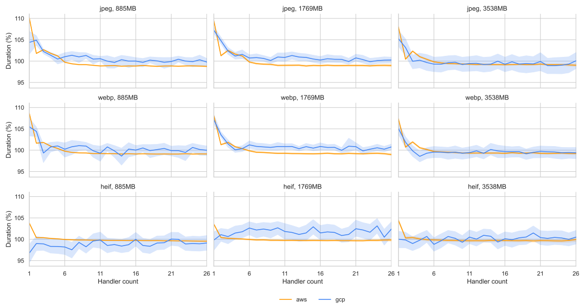
Figure 4.21: Average image processing duration in different variants by handler count.
