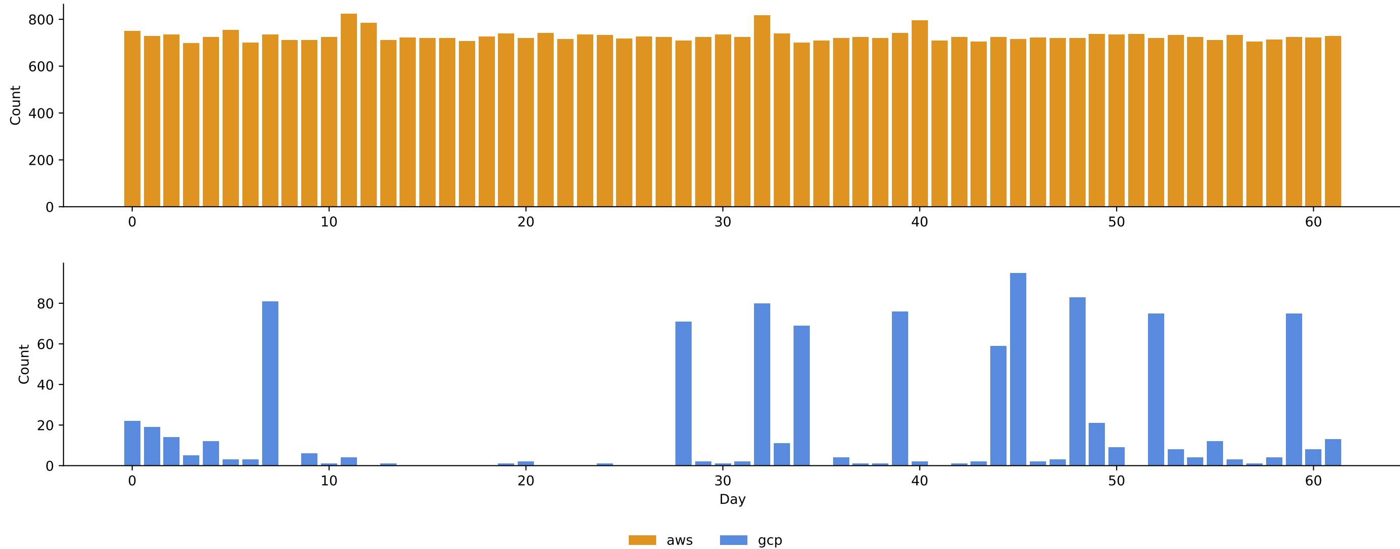
Cold starts per provider, by Day
