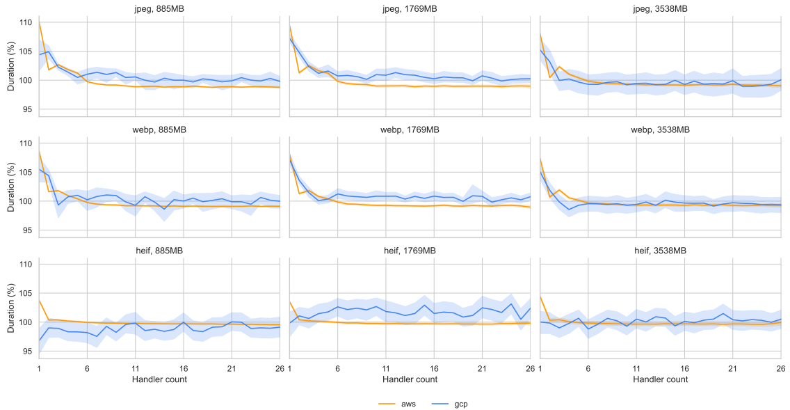
Figure 4.17: Average image processing duration in different variants by handler count.
