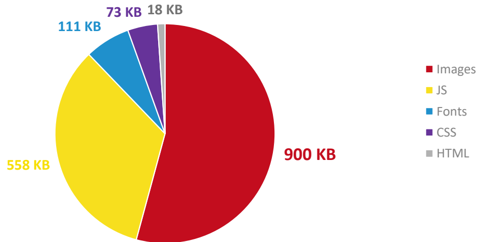
Figure 2.1: Median mobile homepage weight, by content type [81]
