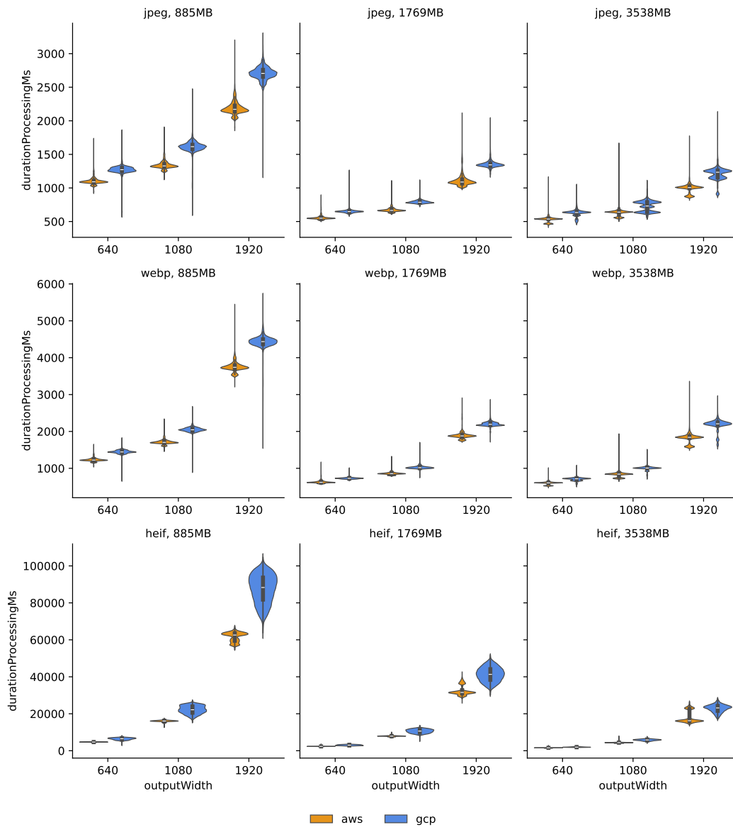
Figure 4.14: Absolute image processing durations, portrait .
