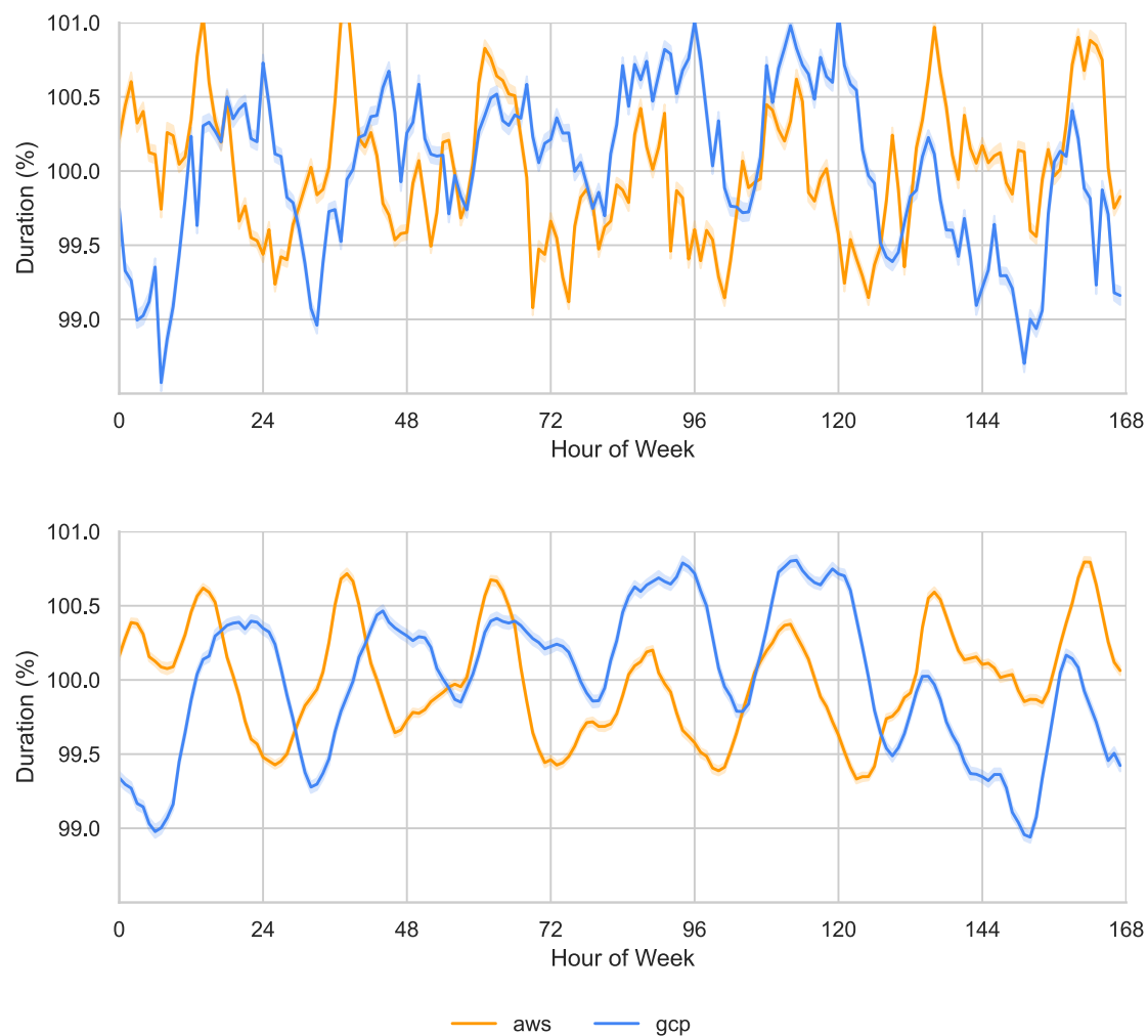
Figure 4.22: Image optimization duration throughout a week: raw aggregated values (above) and smoothened aggregate based on a rolling average (below).
