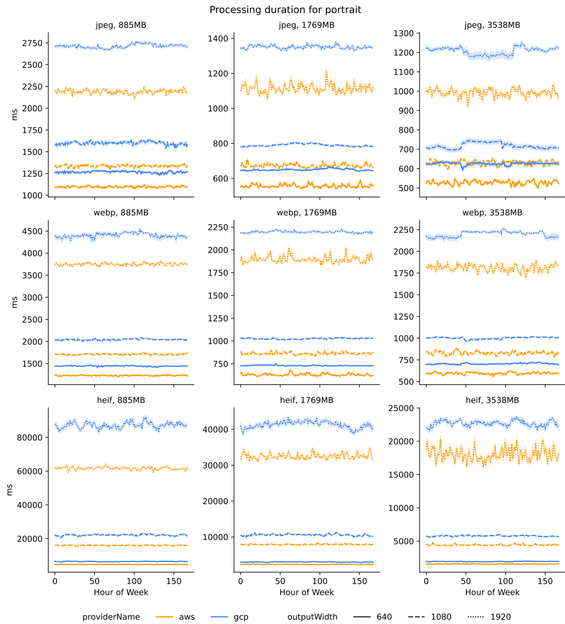
Figure 4.15: Absolute image processing durations by hour of week.
