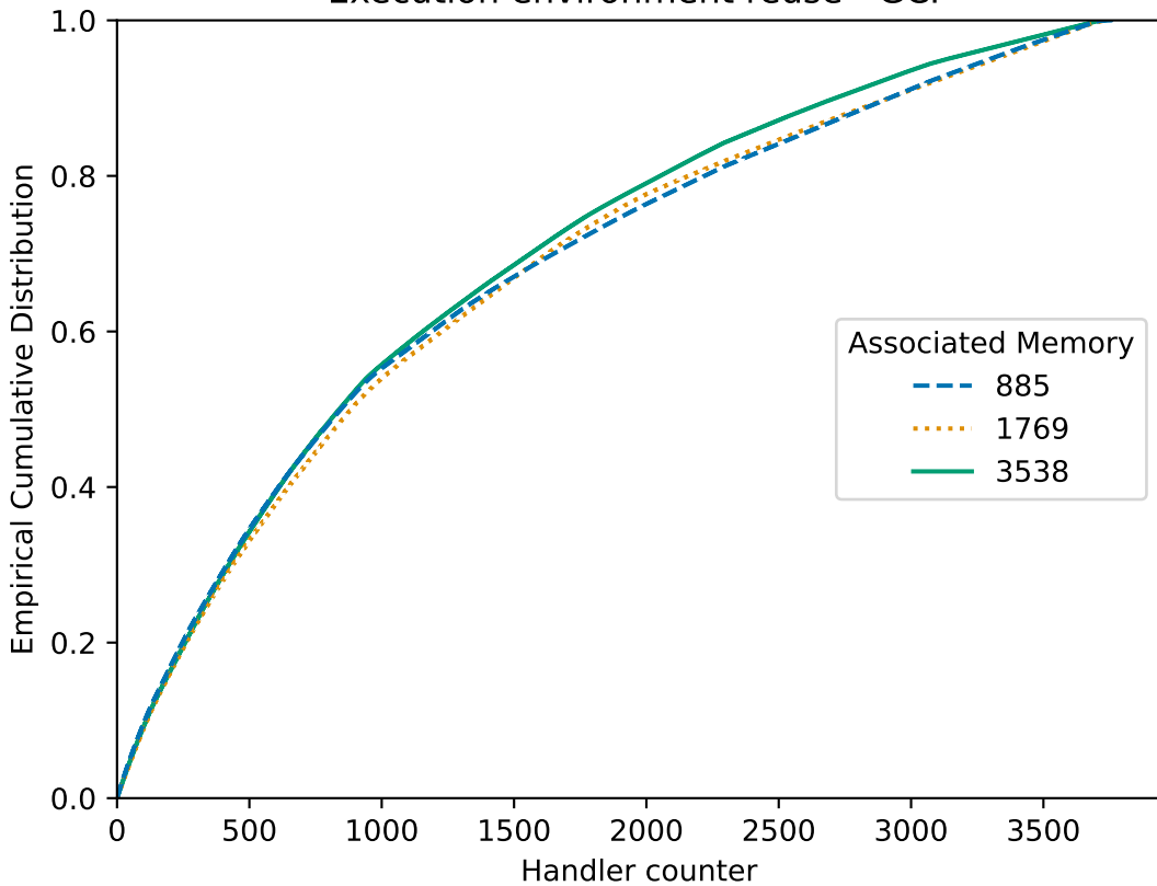
Execution environment reuse - GCP
