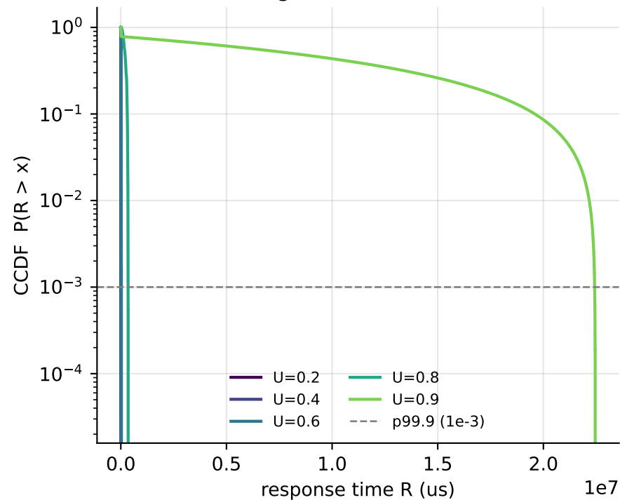
Model 1 — response-time tail (CCDF) [tb-20260708-1113]
