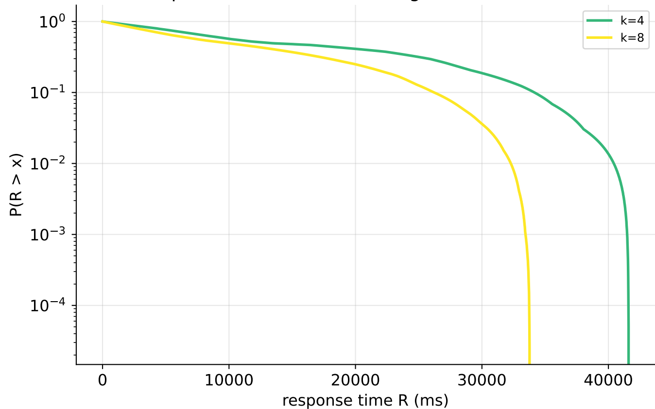
Intra per-task R CCDF vs k — tight (P=10 ms) U=0.2
