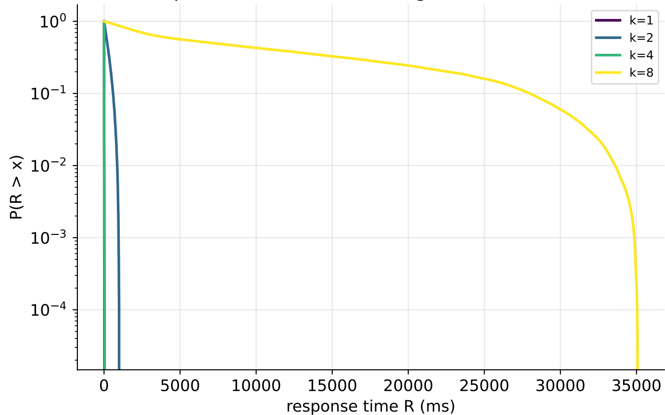
Intra per-task R CCDF vs k — tight (P=10 ms) U=0.4
