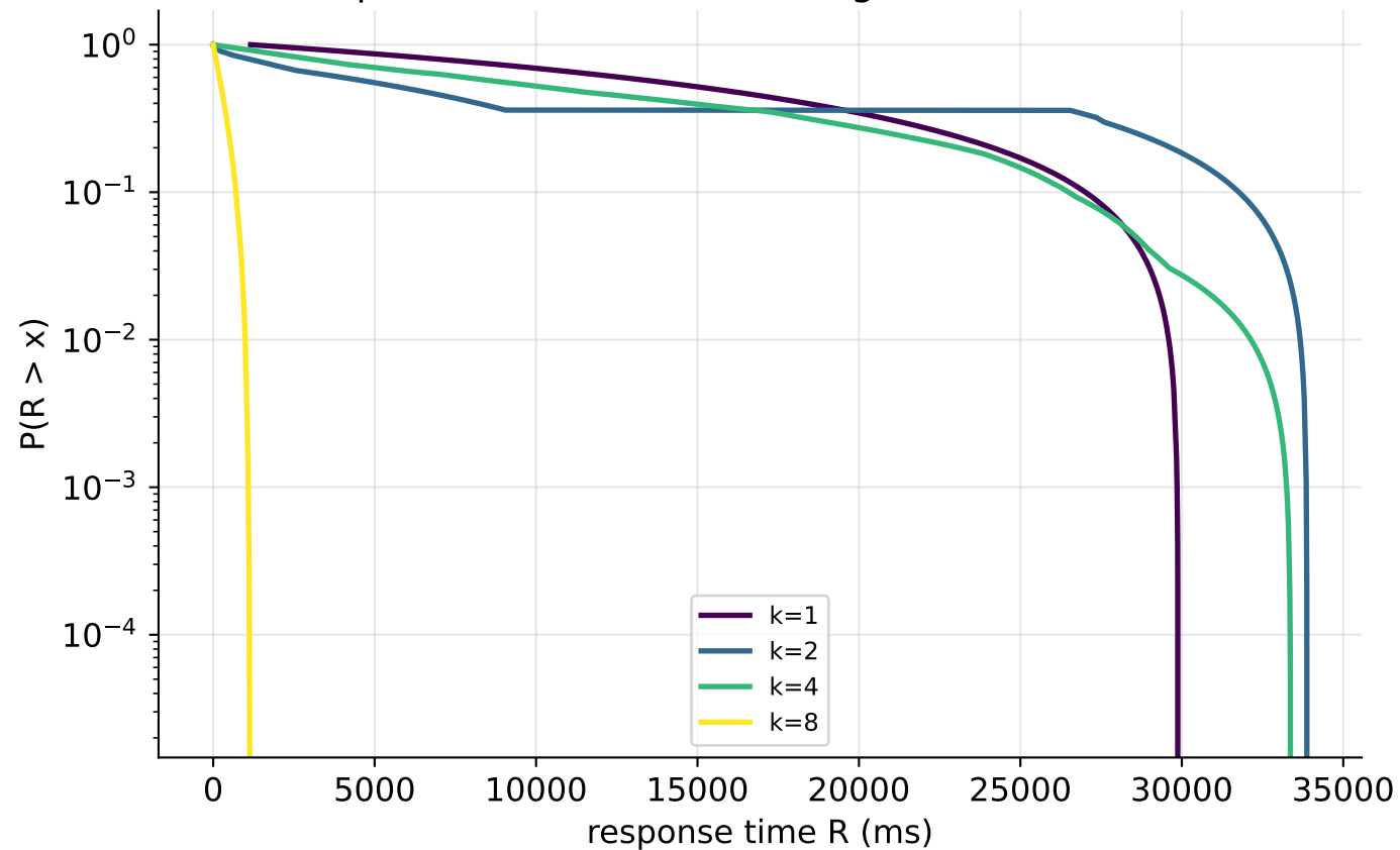
Intra per-task R CCDF vs k — tight (P=10 ms) U=0.6
