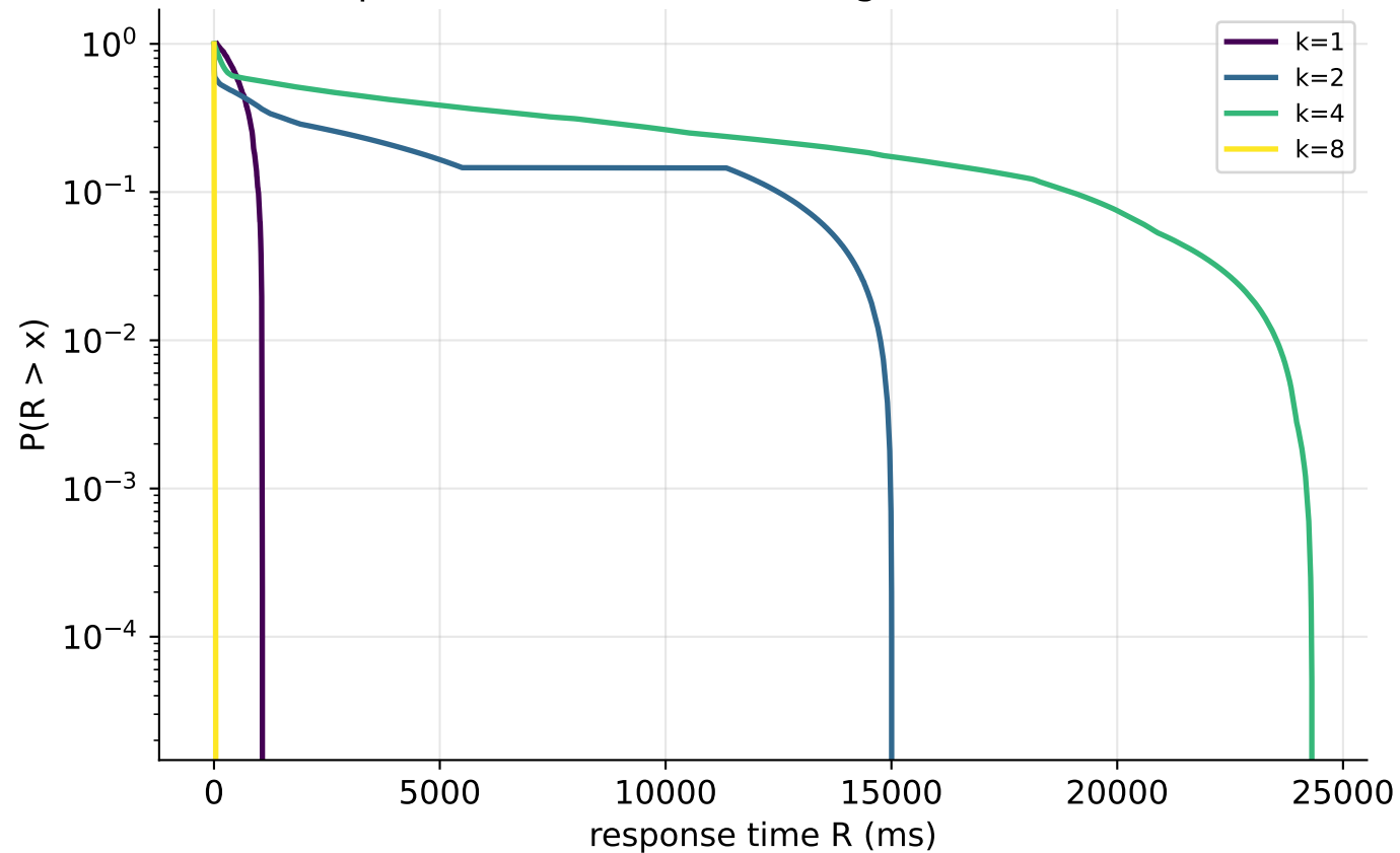
Intra per-task R CCDF vs k — tight (P=10 ms) U=0.8
