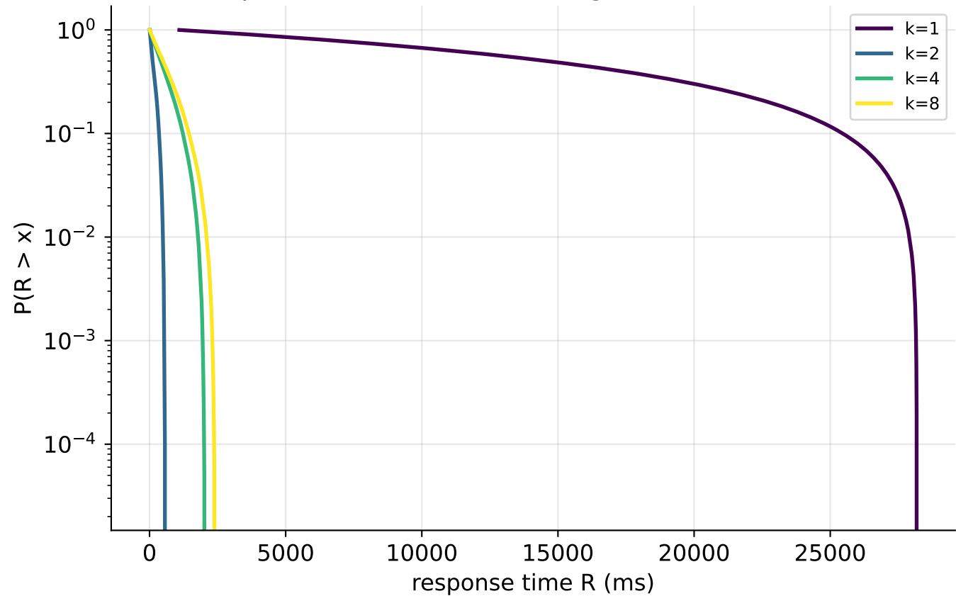
Intra per-task R CCDF vs k — tight (P=10 ms) U=0.94
