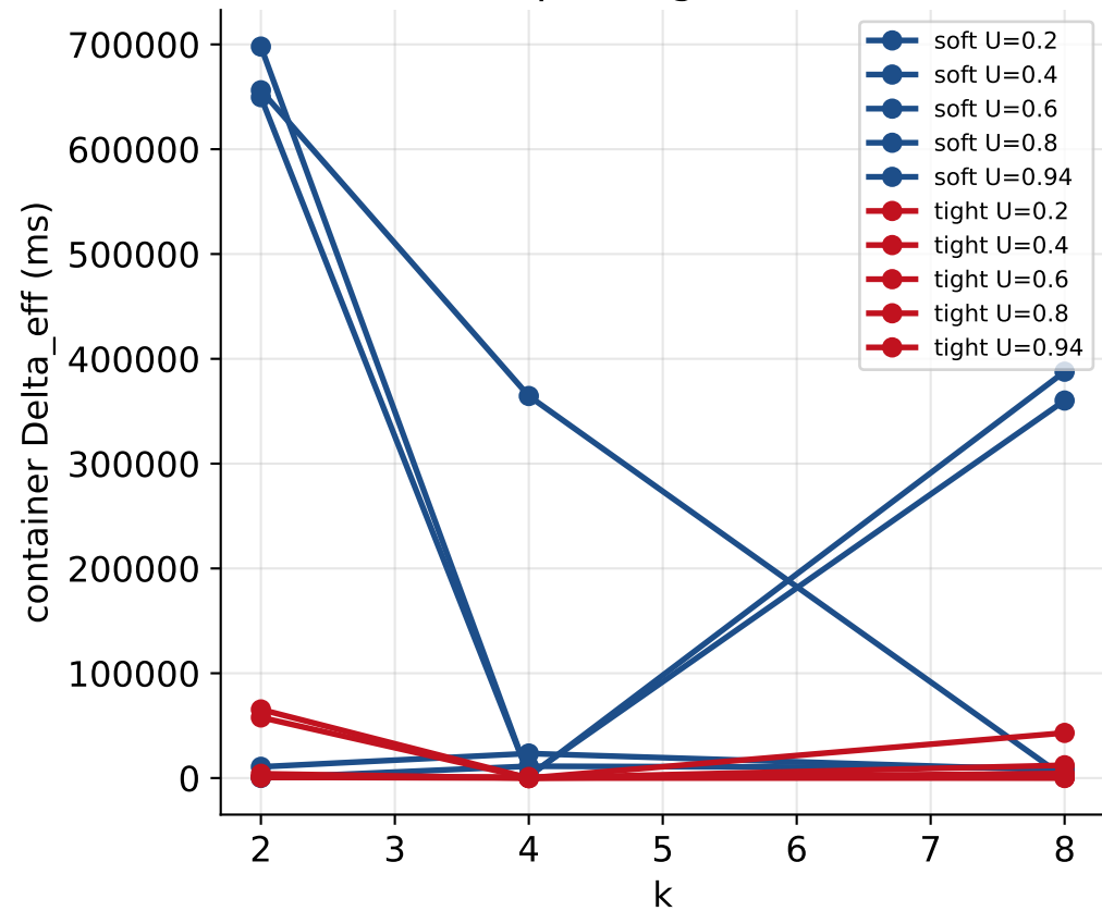
Intra (victim split): Delta_eff & alpha_eff vs k inner spread grows with k
