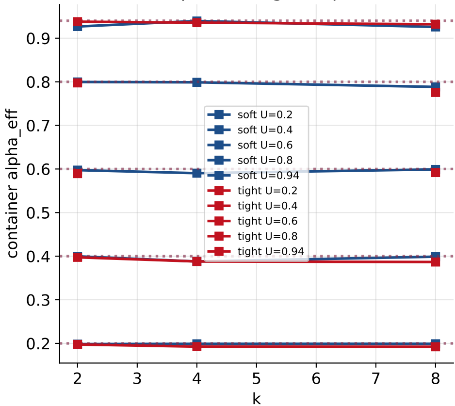
Intra (victim split): Delta_eff & alpha_eff vs k inner spread grows with k
